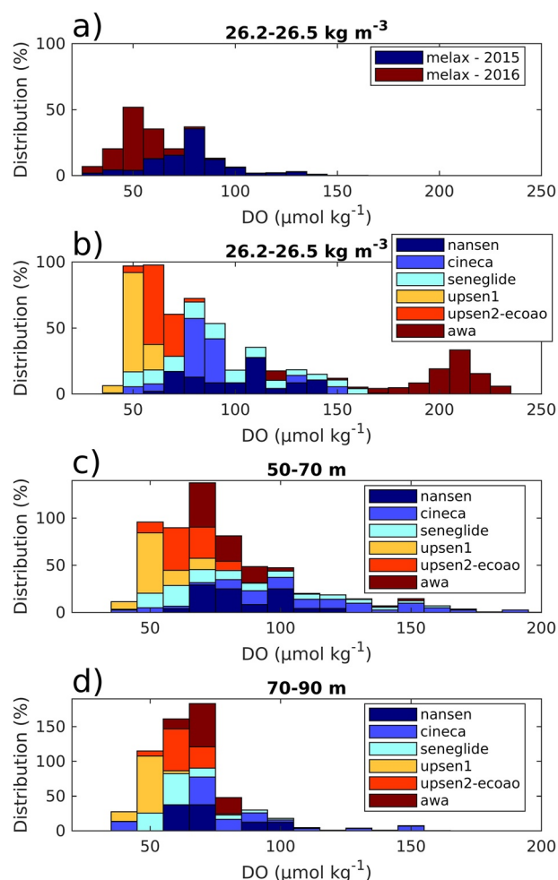
Figure 9. (a) Distribution of dissolved oxygen (DO) concentrations measured in the 26.2–26.5 \text{kg m}^{-3} density range during the upwelling seasons of 2015 and 2016 at Melax. Melax data are compared to (b) prior measurements collected during NANSSEN (dark blue), CINECA (light blue), SENEGLIDE (sky blue) UPSEN1 (orange), UPSEN2-ECOAO (red), and AWA (brown) field experiments in the same density range. (c and d) indicate the DO concentrations from field experiments in two depth ranges. The locations where the data were taken are indicated in Figure 1. Except for the Melax data, all observations are from upper slope waters offshore of the shelf break.
