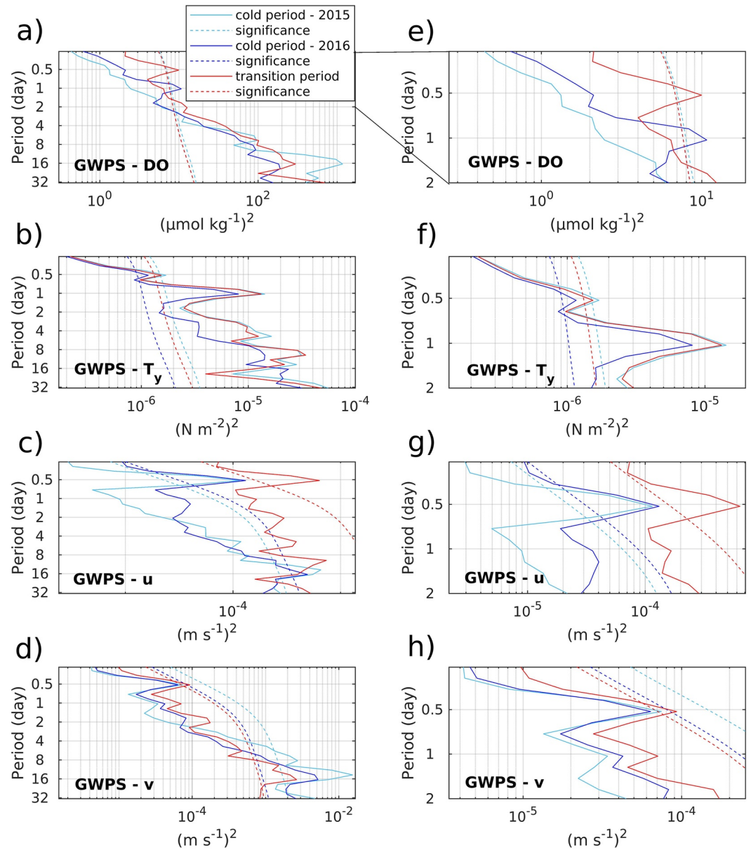
Figure 4. Global wavelet power spectra (GWPS) using Morlet's wavelet (i.e., Torrence & Campo, 1998) of (a) dissolved oxygen (DO), (b) meridional wind stress, (c) zonal and (d) meridional current velocities. (e–h) are zooms of panels (a–d) respectively for times scales shorter than 2 days. GWPS are shown in light blue (dark blue) for the cold periods of 2015 (2016) and in red for the transition from warm to the cold season. The dotted curves represent the significance thresholds of the corresponding spectra.
