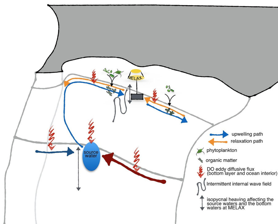
Figure 8. Schematic representation of the processes relevant to the dissolved oxygen (DO) dynamics over the southern Senegalese upwelling sector during the period January–February to April–May when equatorward circulation dominates over the shelf. Upwelling brings cold DO poor slope water onto the shelf following a relatively stable path that hugs the southern part of the Cape Verde peninsula. These source waters (which belong to the South Atlantic Central Water class) are drawn onto the shelf from a depth range that varies depending on local and remote conditions. They are typically brought to the Senegalese slope area by the West African boundary current but slope current variability and the existence of regional-scale DO gradients off West Africa implies that their properties can vary on synoptic and seasonal scales (see Section 4.3 for details). Vertical mixing can also impact source waters DO levels in high wind-low air-sea heat flux conditions in which the surface boundary layer turbulence reaches down to typical source water depths. Isopycnal heaving can also affect the properties of upwelling source waters. On their path to Melax, upwelling waters DO concentration can be modified by organic matter degradation and mixing. In relaxation conditions the shelf circulation tends to reverse to poleward and old upwelling waters previously advected southward may recirculate northward at Melax.
