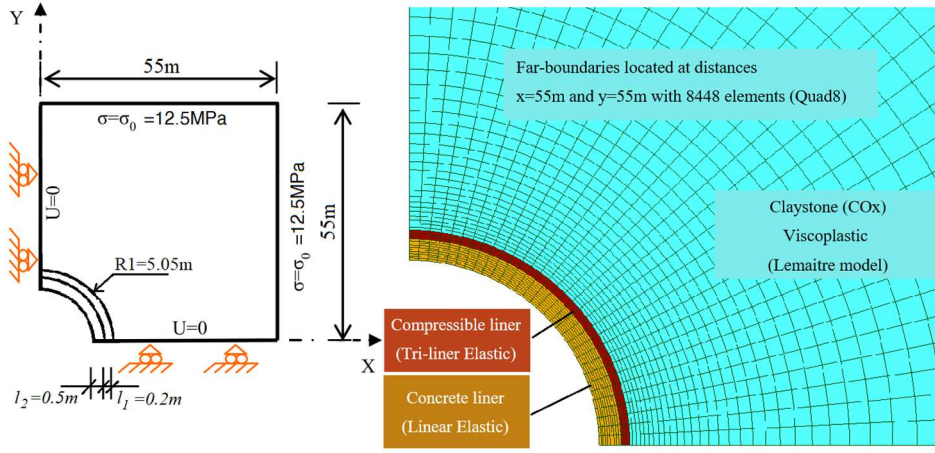
Fig. 1. 2D plane strain model of drift supported by the outer compressible and inner concrete liners in viscoplastic COx rock.
