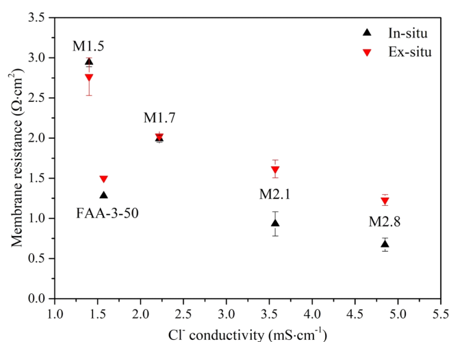
Figure 5. Membrane resistances compared to their chloride ion conductivity.
