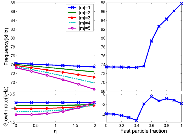
Figure 3: Evolution of the BAE frequency and growth rate with the temperature gradient, and fraction of fast particles.
