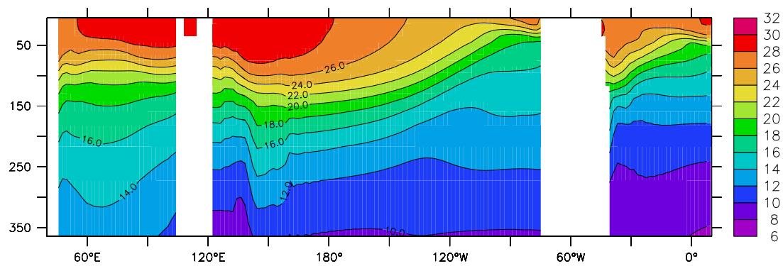
LJ7 Temperature
