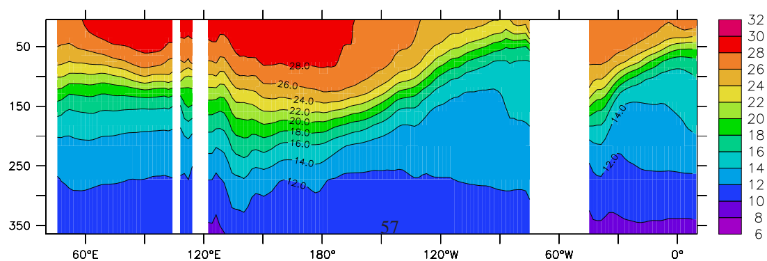
Levitus Temperature
