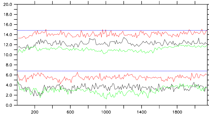
Figure 4.9: Sea ice surface : yearly maxima and minima for northern hemisphere in 10^6 km^2 . Black: LJ7, red: 2L20 and green: BR01. Blue lines are observations ( Gloersen and Campbell, 1991 ). Time axis in month.
