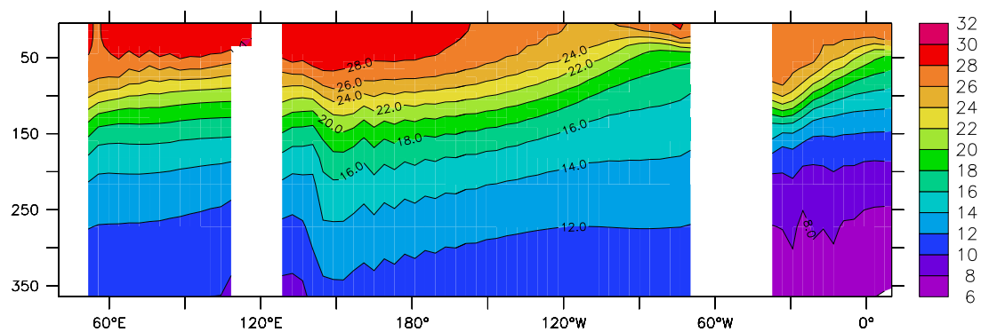
BR01 Temperature
