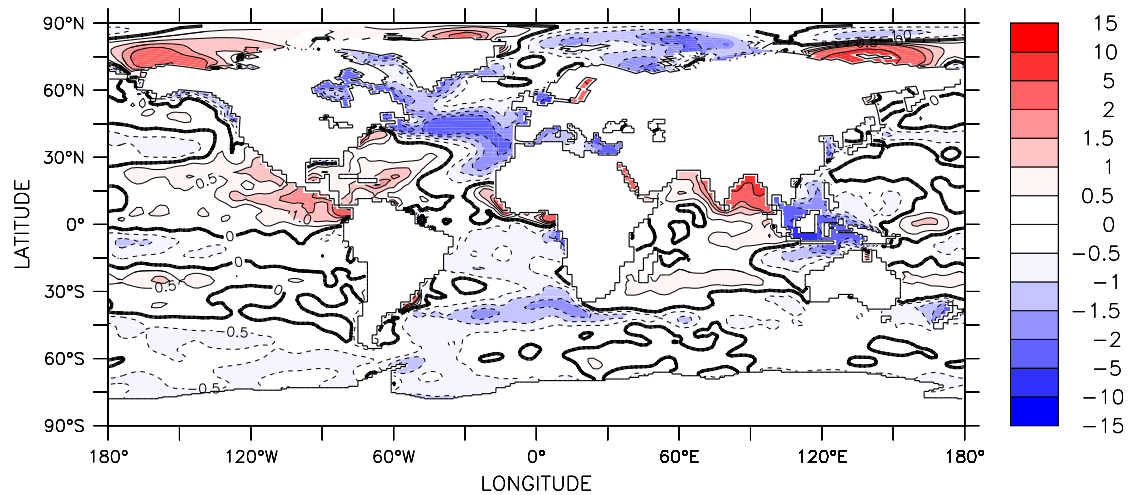
Figure 4.16: Sea surface salinity. Difference between 2L20 and Levitus (1982) data. Contour interval 0, \pm 0.5 , \pm 1 , \pm 1.5 , \pm 2 , \pm 5 , \pm 10 and \pm 15 PSU.
