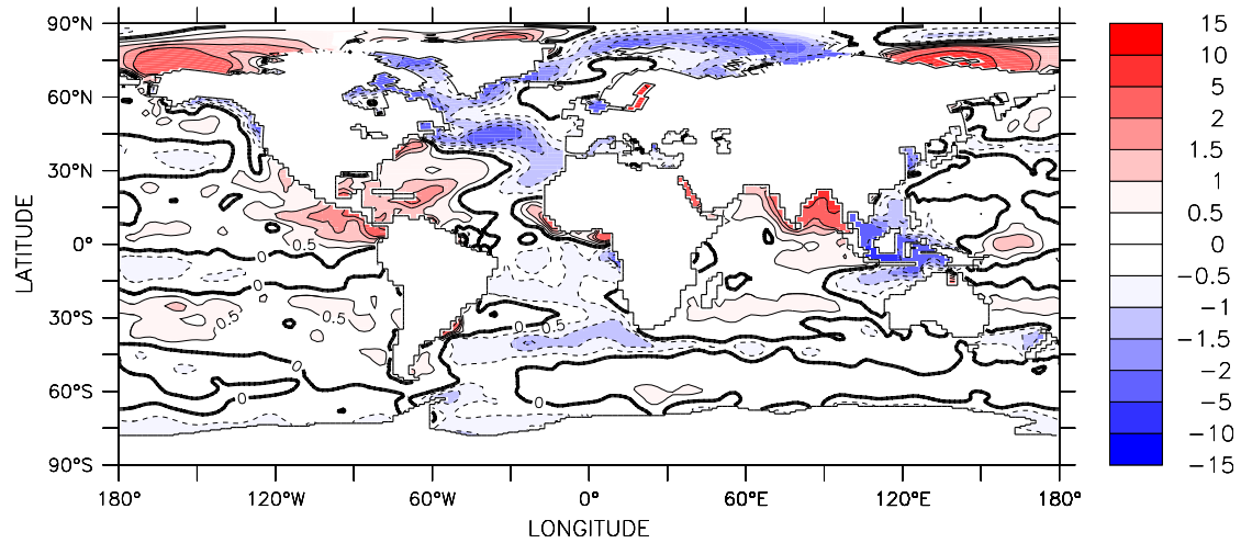
Figure 4.15: Sea surface salinity. Difference between LJ7 and Levitus (1982) data. Contour interval 0, \pm 0.5 , \pm 1 , \pm 1.5 , \pm 2 , \pm 5 , \pm 10 and \pm 15 PSU.
