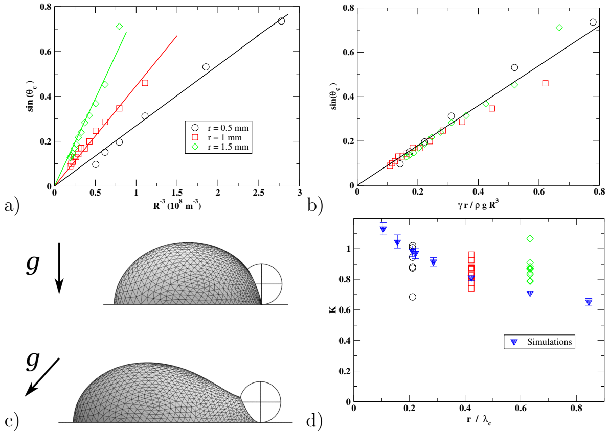
FIG. 2. K -analysis in experiments and simulation. a) \sin(\theta_c) as a function of R^{-3} in experiments for beads of radius 0.5 (black circles), 1 (red squares) and 1.5 mm (green diamonds). Proportionality relations are displayed by solid lines. b) Same data with \sin(\theta_c) as a function of \gamma r / (\rho g R^3) with \gamma = 55 \text{ mN.m}^{-1} . c) Snapshots from the simulation for \theta = 0 and 42^\circ respectively. d) K as a function of r/\lambda_c for both experiments and simulations. In simulation, each point corresponds to one value of r/\lambda_c and roughly 100 values of R/\lambda_c , whose effect is quantified by the error bars.
