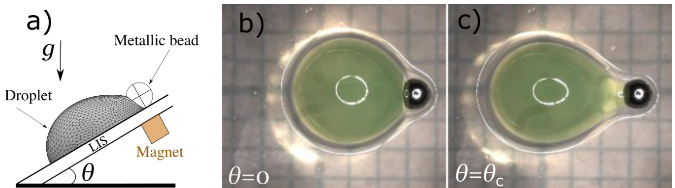
FIG. 1. a) Representation of the system on an inclined plane. Two images taken from above in the reference frame of the substrate for \theta = 0 (b) and at the critical inclination \theta_c (c) respectively ( r = 0.5 mm and R = 2 mm).
