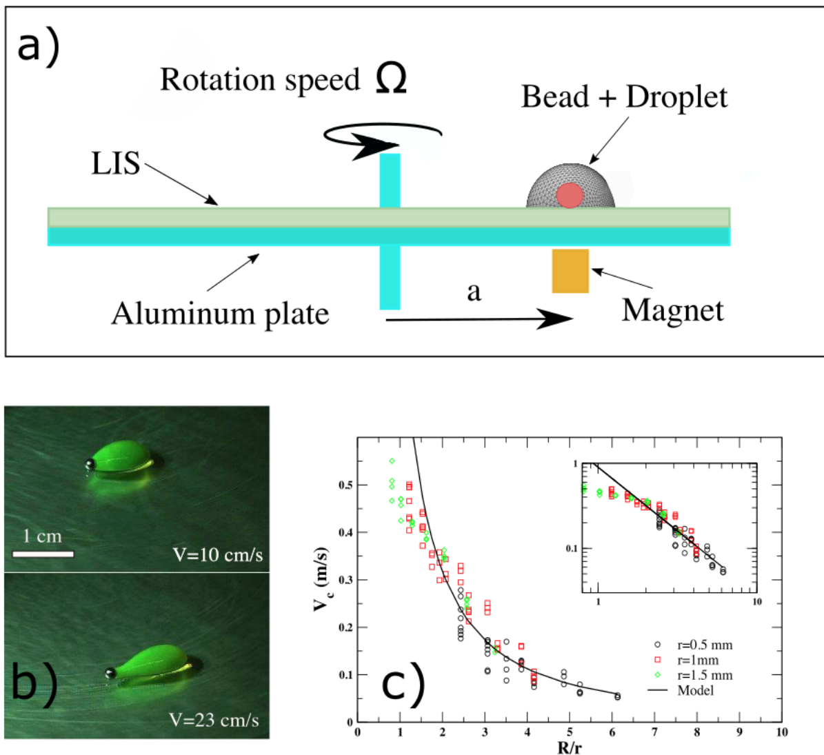
FIG. 3. a) Rotating setup designed to determine the critical velocity. b) Snapshots taken for two velocities (the lower one is taken just prior to detachment). c) Critical velocity V_c as a function of R/r . Inset: log-log scale. The solid line is a power law interpolation (exponent -3/2 , prefactor 0.85 \text{ m}\cdot\text{s}^{-1} ).
