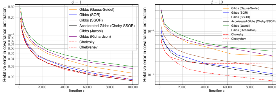
Fig. 10: Scenario 2. Relative error associated to the estimation of the covariance matrix \mathbf{Q}^{-1} defined by \|\mathbf{Q}^{-1} - \text{var}(\boldsymbol{\theta}^{(1:t)})\|_2 / \|\mathbf{Q}^{-1}\|_2 w.r.t. the number of iterations t in Algorithm 4.2 , with d = 100 (left: \phi = 1 , right: \phi = 10 ). We also highlighted the relative error obtained with an increasing number of samples generated independently from Cholesky and Chebyshev samplers. The results have been averaged over 30 independent runs. The standard deviations are not shown for readability reasons.
