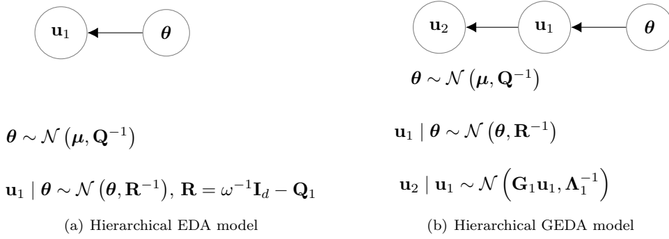
Fig. 4: Hierarchical models proposed in [66,67] where \omega is such that 0 < \omega < \|\mathbf{Q}_1\|^{-1} .
