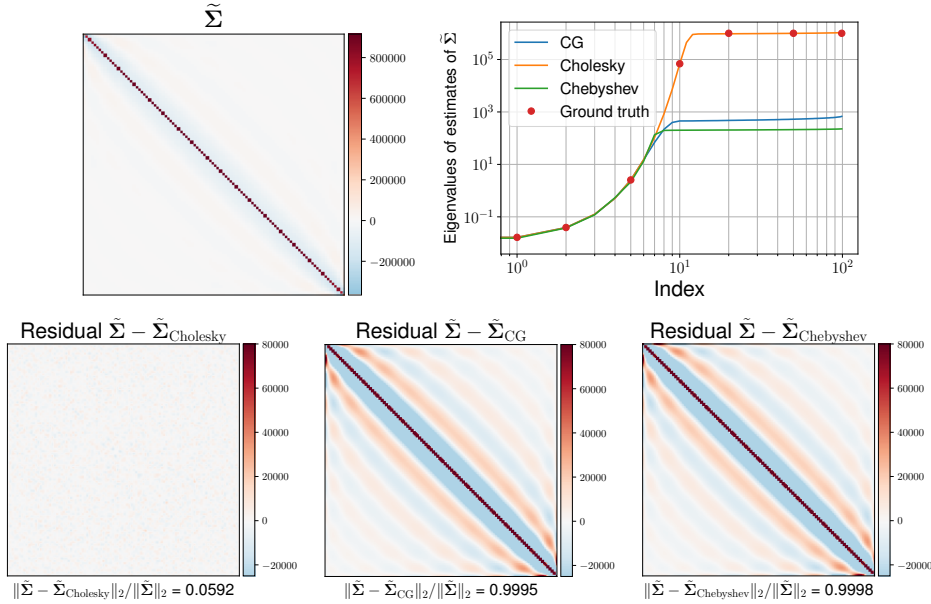
Fig. 7: Scenario 1. Results of the three considered samplers for the sampling from \mathcal{N}(\mathbf{0}_d, \tilde{\Sigma}) in dimension d = 100 .
