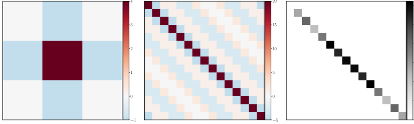
Fig. 2: From left to right: example of a 3 \times 3 Laplacian filter, the associated circulant precision matrix \mathbf{Q} = \mathbf{\Delta}^\top \mathbf{\Delta} for convolution with periodic boundary conditions and its counterpart diagonal matrix \mathbf{F}\mathbf{Q}\mathbf{F}^\mathbf{H} in the Fourier domain, where \mathbf{F} and its Hermitian conjugate \mathbf{F}^\mathbf{H} are unitary matrices associated with the Fourier and inverse Fourier transforms.
