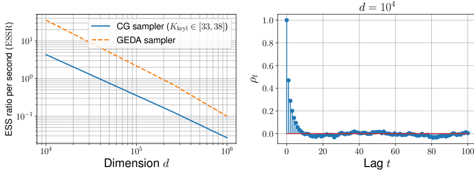
Fig. 11: Scenario 3. (left) ESS ratio per second (ESSR); (right) autocorrelation function \rho_t shown for d = 10^4 . For both figures, we used the slowest component of \boldsymbol{\theta} as the scalar summary \vartheta .
