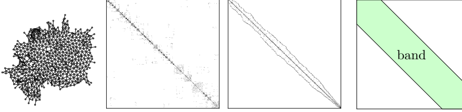
Fig. 1: From left to right: example of an undirected graph defined on the 544 regions of Germany where those sharing a common border are considered as neighbors, its associated precision matrix \mathbf{Q} (bandwidth b = 522 ), its re-ordered precision matrix \mathbf{PQP}^\top ( b = 43 ) where \mathbf{P} is a permutation matrix and a drawing of a band matrix. For the three matrices, the white entries are equal to zero.
