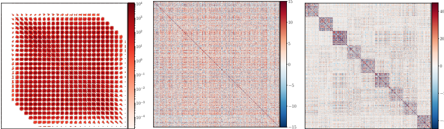
Fig. 3: Examples of precision matrices \mathbf{X}^\top \mathbf{X} for three datasets. Left: MNIST dataset [57]. Only the predictors associated to the digits 5 and 3 have been taken into account for the MNIST dataset [57]. Middle: leukemia dataset [6]. For the leukemia dataset [6], only the first 5,000 predictors (out of 12,600) have been taken into account. Right: CoEPrA dataset [52].
