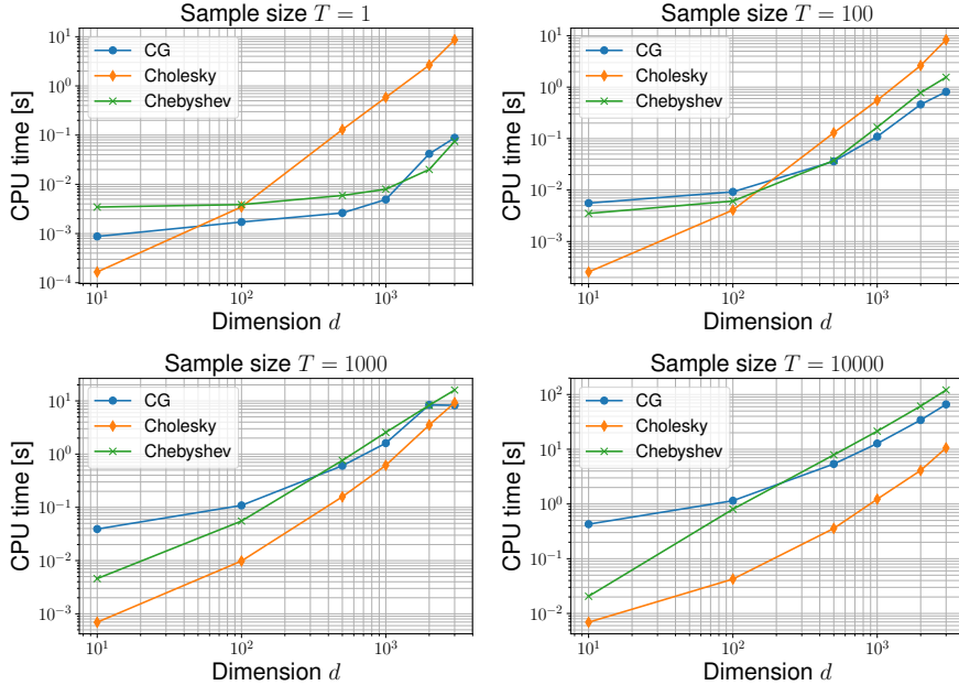
Fig. 6: Scenario 1. Comparison between the three considered direct samplers in terms of CPU time for the sampling from \mathcal{N}(\mathbf{0}_d, \Sigma) with \Sigma detailed in (6.2).
