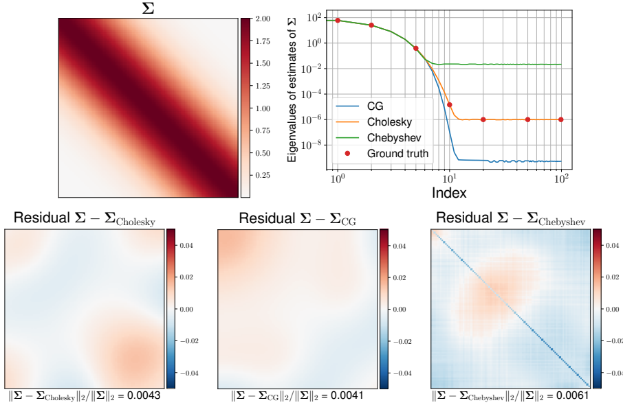
Fig. 5: Scenario 1. Results of the three considered samplers for the sampling from \mathcal{N}(\mathbf{0}_d, \Sigma) in dimension d = 100 with \Sigma detailed in (6.2).
