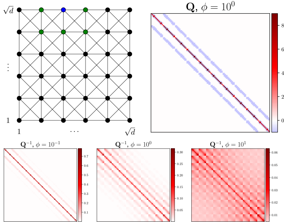
Fig. 9: Scenario 2. Illustrations of considered the Gaussian sampling problem: (top left) 2D-lattice ( d = 36 ) associated to the precision matrix \mathbf{Q} in (6.3), (top right) \mathbf{Q} depicted for \phi = 1 and (bottom) \mathbf{Q}^{-1} = \Sigma for \phi \in \{0.1, 1, 10\} . All the results are shown for d = 100 . On the 2D-lattice, the green nodes stand for the neighbors of the blue node while the coordinates of the lattice correspond to the coordinates of \boldsymbol{\theta} \in \mathbb{R}^d with non-zero correlations, that is 1 \leq i, j \leq \sqrt{d} .
