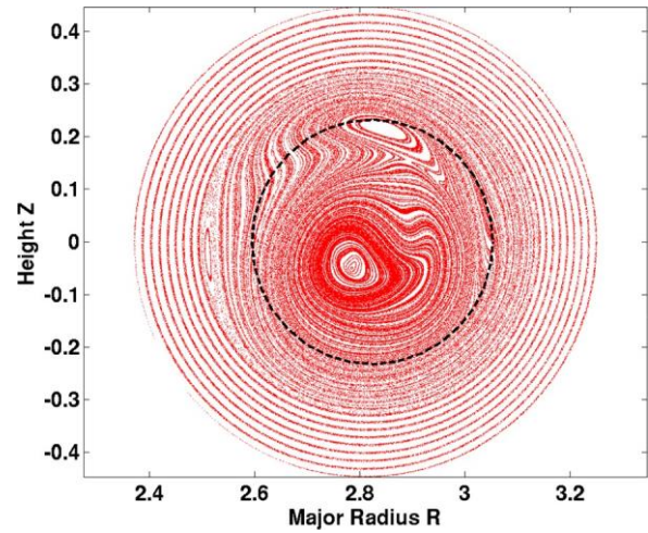
FIG. 8. Poincaré plot at the end of the reconnection phase. The small remainder of the reconnecting core can be observed at the left of the figure, well beyond the initial q/4 surface location (dashed circle), at a location corresponding to the mixing radius.
