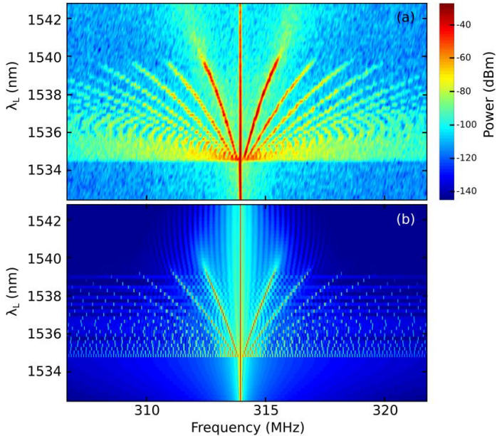
FIG. 3: Evolution of the electro-optomechanical modulation instability radio-frequency spectrum as function of the driving laser wavelength. (a) Experiment. (b) Theory.
