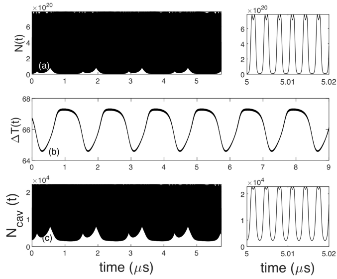
FIG. 6: Time evolution of the variables involved in the electro-optomechanical instability. (a) Free-carrier density, (b) Temperature elevation, (c) Intracavity photon number, as a function of time. Time traces are calculated from the model introduced in the main text, under the conditions of Fig. 3.
