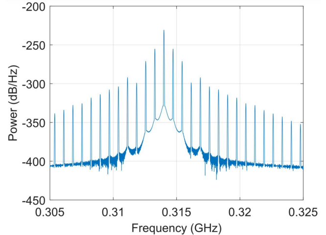
FIG. 5: Mechanical comb controlled by light. Spectrum of the pulsing mechanical motion shown in Fig. 4c of the main text, obtained by Fast Fourier Transform using a Kaiser window.
