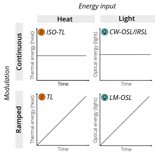
Figure 3: Stimulation modes in RLucCarlo applicable to the models. ISO-TL: isothermal TL, i.e., constant stimulation temperature over time. TL: thermal luminescence, i.e., temperature ramps (approximately linearly) over time. CW-OSL/IRSL: continuous wave optically stimulated luminescence respectively infrared stimulated luminescence, constant optical stimulation over time. LM-OSL: linearly modulated optically stimulated luminescence, i.e., linearly ramped optical stimulation over time.
