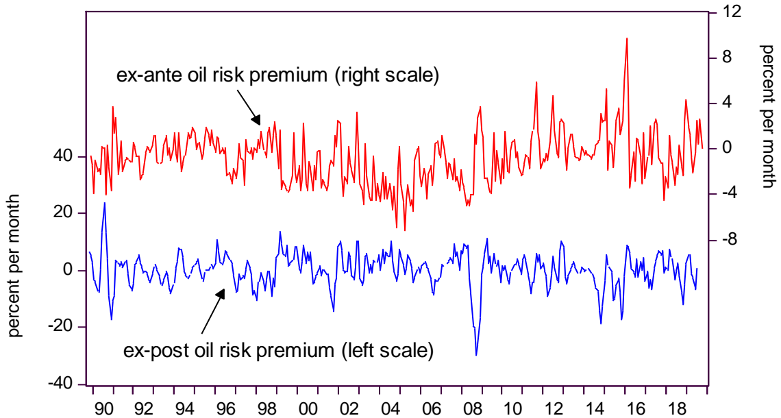
Figure 3. Ex-ante and ex-post 3-month horizon crude oil risk premia
