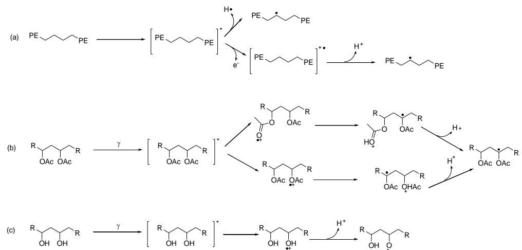
Scheme 1. Generation of radicals from PE (a), PVA (b), and PVOH (c).
