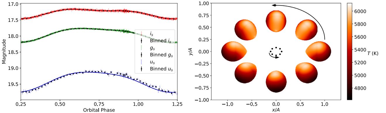
Figure 9. Left: i_s , g_s , and u_s light curves of J1023 overlaid with the best-fitting hotspot model with 40 phase bins in black. Right: temperature distribution of companion, showing the asymmetry which manifests as a large polar spot. The dark band around the star is an artefact due to the plotting only.
