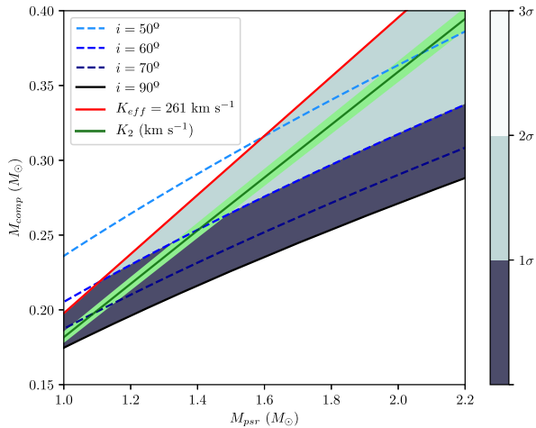
Figure 8. The mass ratio calculated from the centre-of-light K_{\text{eff}} value, in red, provides us with a lower limit of the pulsar mass for each inclination, while the best-fitting mass ratio from each fit’s K_2 is in green. The binary mass function at each inclination is shown by the series of blue dashed lines, with the absolute limit at i = 90^\circ shown by a solid black line. As such, the excluded region of the mass–mass plot is in white. The best-fitting model distance at each inclination is interpolated over the mass–mass plane. The shaded area then represents the corresponding confidence interval of the distances with respect to the distance prior.
