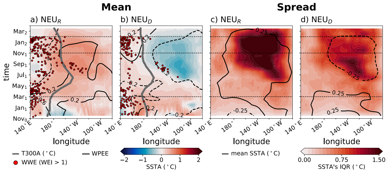
FIG. 5. Time section of the 70-member ensemble experiments starting on 1 November 0 from neutral ENSO states, with either a recharged ( NEU_R ) or discharged ( NEU_D ) T300 W A. (a), (b) 5°N–5°S meridional averaged ensemble mean SSTA (shading; °C) and T300A (black contours; °C), WPEE (gray line), and WWE from all 70 members with a WEI index above 1 (red dots). (c), (d) The 5°N–5°S meridional averaged ensemble IQR of SSTA (shading; °C) and ensemble mean SSTA (black contours; °C). The NEU_R and NEU_D experiments correspond to initial states respectively marked by the dark red and dark turquoise crosses on Fig. 3c. Data are smoothed with an 11° and 3-months triangular-weighted running average prior to plotting.
