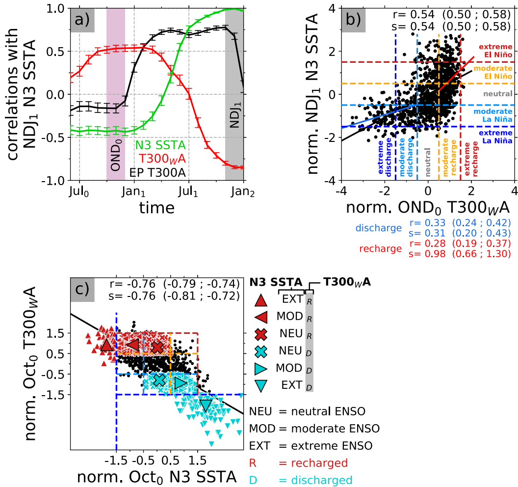
FIG. 3. (a) Lead correlations between T300_{WA} (red), anomalies of T300 averaged over the entire equatorial Pacific (EP T300_A ; black), N3\ SSTA (green), and NDJ_1 (gray shading) N3\ SSTA . Error bars indicate the 95% confidence interval. (b) Scatterplot of normalized NDJ_1 [gray shading in (a)] N3\ SSTA vs normalized OND_0 [purple shading in (a)] T300_{WA} . (c) Scatterplot of normalized October 0 T300_{WA} vs normalized October 0 N3\ SSTA . This figure is used to select initial states for our ensemble predictability experiments. In (b) and (c), the dashed lines indicate the -1.5 \times STD (deep blue; limit between extreme and moderate La Niña/discharges), -0.5 \times STD (light blue; limit between moderate and neutral La Niña/discharges), 0.5 \times STD (orange; limit between neutral and moderate El Niño/recharge), and 1.5 \times STD (red; limit between moderate and extreme El Niño/recharge) thresholds. In (b) and (c), the black solid line represents the linear regression slope, and the corresponding r and s are indicated at the top of each panel, with the 95% confidence interval within brackets. In (b), the blue and red solid lines represent the linear regression slopes computed for discharged and recharged states, and the corresponding r and s are indicated under the panel, with the 95% confidence interval within parentheses. The CNRM-CM5 1007-yr-long control experiment is used for this figure.
