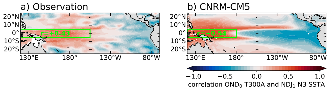
FIG. A1. Spatial structure of the correlation between OND 0 T300A and NDJ 1 N3 SSTA computed with (a) observations and (b) CNRM-CM5. Limits of the western equatorial Pacific region used for the observations and CNRM-CM5 are outlined in green. The correlation between OND 0 T300 WA and NDJ 1 N3 SSTA is indicated in the box.
