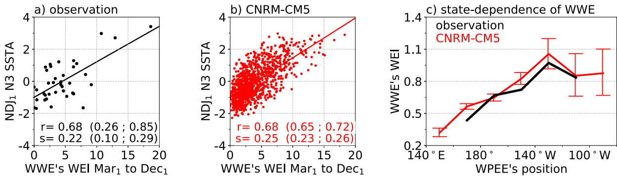
FIG. 2. Scatterplots of ENSO peak amplitude (NDJ1 N3 SSTA) vs March–December total WEI index for (a) observations and (b) CNRM-CM5. Solid lines represent the linear regression slopes. The corresponding correlation r and regression slope s are indicated at the bottom of each panel, with the 95% confidence interval in parentheses. (c) WEI as a function of the WPEE position for observations (black) and CNRM-CM5 (red), indicative of the state-dependent component of WWE. The WEI is summed across longitudes for each month and averaged for a given position of the WPEE ( 20^\circ bins). Red error bars indicate the 95% confidence interval computed with CNRM-CM5 (the confidence interval is larger for the observations and for readability is not plotted).
