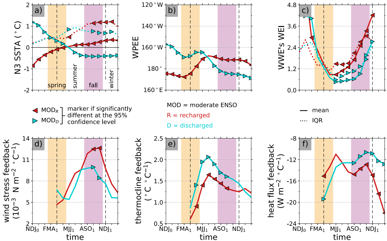
FIG. 7. As in Fig. 6, but for 70-member ensemble experiments starting on 1 November 0 from either a moderate La Niña recharged T300 wA (MOD R ; dark red) or a moderate El Niño discharged T300 wA (MOD D ; dark turquoise). The MOD R and MOD D experiments respectively correspond to initial states marked by the dark-red left-pointing triangles and dark-turquoise right-pointing triangles in Fig. 3c.
