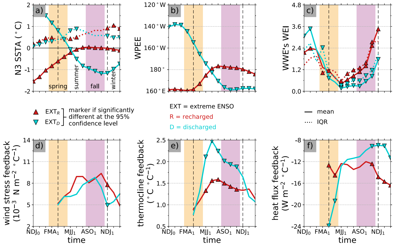
FIG. 8. As in Fig. 6, but for 70-member ensemble experiments starting on 1 November 0 from either an extreme La Niña recharged T300 WA (EXT R ; dark red) or an extreme El Niño discharged T300 WA (EXT D ; dark turquoise). The EXT R and EXT D experiments respectively correspond to initial states marked by the dark-red upward-pointing and dark-turquoise downward-pointing triangles in Fig. 3c.
