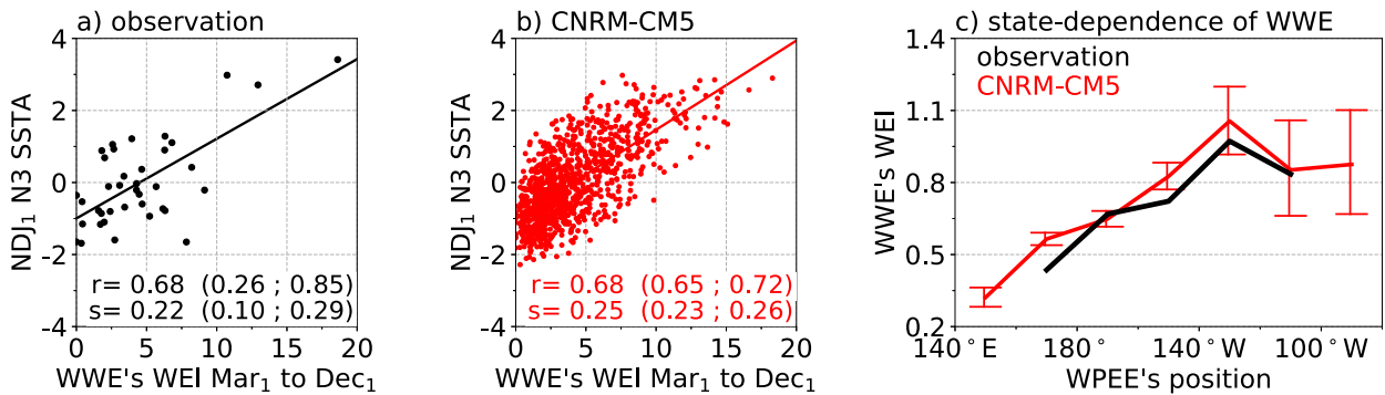
FIG. 2. Scatterplots of ENSO peak amplitude (NDJ 1 N3 SSTA) vs March 1 –December 1 total WEI index for (a) observations and (b) CNRM-CM5. Solid lines represent the linear regression slopes. The corresponding correlation r and regression slope s are indicated at the bottom of each panel, with the 95% confidence interval in parentheses. (c) WEI as a function of the WPEE position for observations (black) and CNRM-CM5 (red), indicative of the state-dependent component of WWE. The WEI is summed across longitudes for each month and averaged for a given position of the WPEE (20° bins). Red error bars indicate the 95% confidence interval computed with CNRM-CM5 (the confidence interval is larger for the observations and for readability is not plotted).
