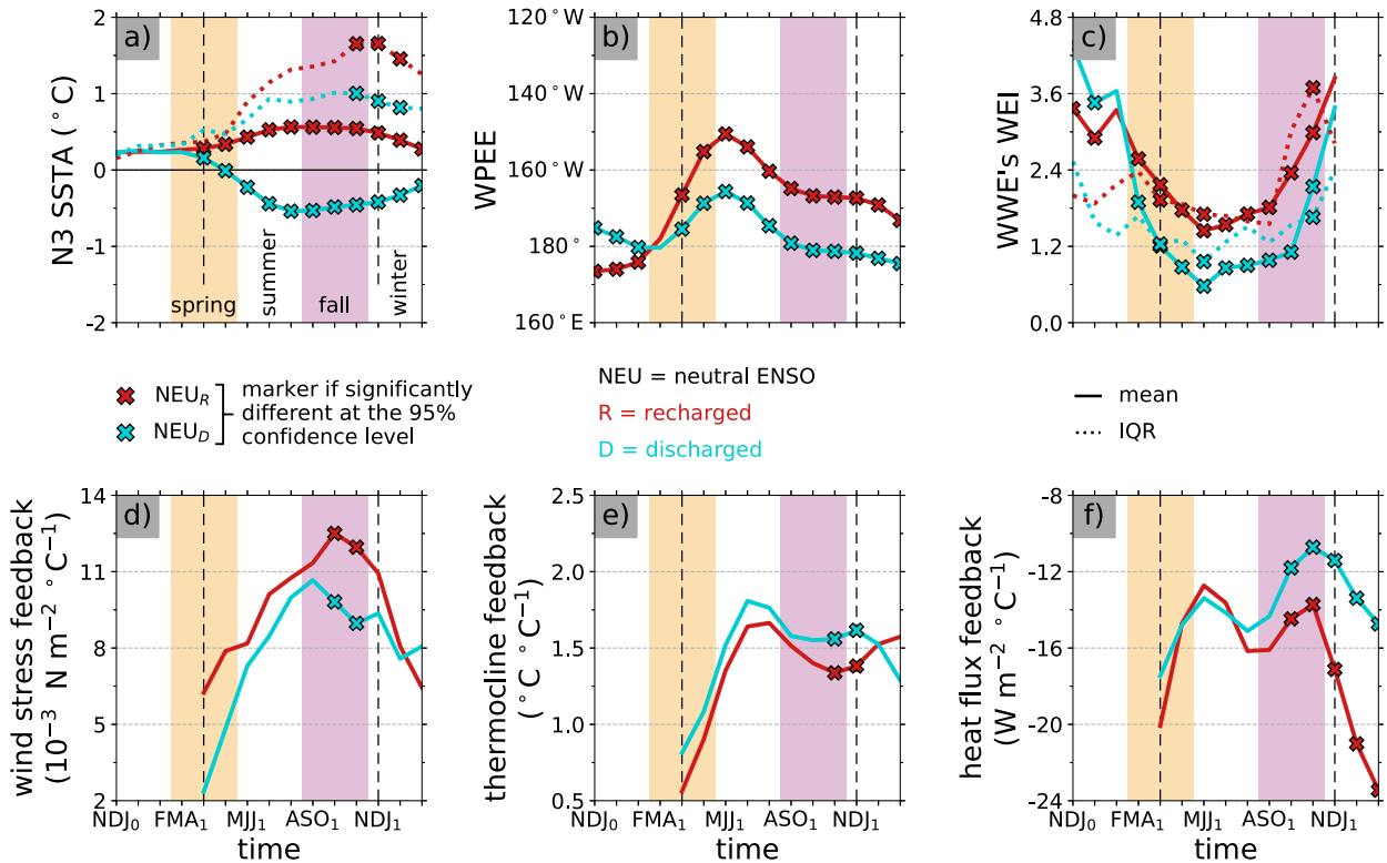
FIG. 6. Evolution of the key ENSO variables and feedbacks in the 70-member ensemble experiments starting on 1 November 0 from a neutral ENSO state, with either a recharged ( NEUR ; dark red) or discharged ( NEUD ; dark turquoise) T300 W A. Ensemble mean (solid line) of (a) N3 SSTA ( ^{\circ}\text{C} ), (b) position of the WPEE, (c) WEI index (seasonally integrated across longitudes), (d) wind stress feedback ( 10^{-3} \text{ N m}^{-2} \text{ }^{\circ}\text{C}^{-1} ), (e) thermocline feedback ( ^{\circ}\text{C } ^{\circ}\text{C}^{-1} ), and (f) heat flux feedback ( \text{W m}^{-2} \text{ }^{\circ}\text{C}^{-1} ). The IQR of N3 SSTA and WEI are respectively also plotted as dotted lines in (a) and (c). The NEUR and NEUD experiments respectively correspond to initial states marked by the dark red and dark turquoise crosses in Fig. 3c. Crosses indicate significantly different values between NEUR and NEUD experiments, at the 95% confidence level.
