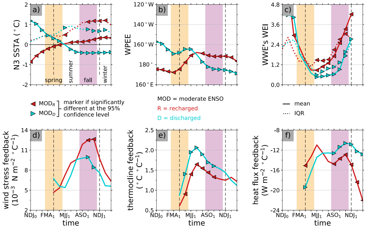
FIG. 7. As in Fig. 6, but for 70-member ensemble experiments starting on 1 November 0 from either a moderate La Niña recharged T300 W A (MOD R ; dark red) or a moderate El Niño discharged T300 W A (MOD D ; dark turquoise). The MOD R and MOD D experiments respectively correspond to initial states marked by the dark-red left-pointing triangles and dark-turquoise right-pointing triangles in Fig. 3c.
