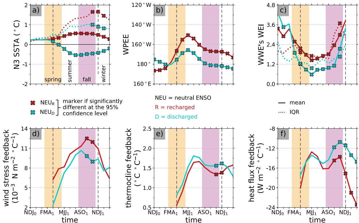
FIG. 6. Evolution of the key ENSO variables and feedbacks in the 70-member ensemble experiments starting on 1 November 0 from a neutral ENSO state, with either a recharged ( NEUR_R ; dark red) or discharged ( NEUR_D ; dark turquoise) T300 W A. Ensemble mean (solid line) of (a) N3 SSTA ( ^{\circ}\text{C} ), (b) position of the WPEE, (c) WEI index (seasonally integrated across longitudes), (d) wind stress feedback ( 10^{-3} \text{ N m}^{-2} \text{ }^{\circ}\text{C}^{-1} ), (e) thermocline feedback ( ^{\circ}\text{C } ^{\circ}\text{C}^{-1} ), and (f) heat flux feedback ( \text{W m}^{-2} \text{ }^{\circ}\text{C}^{-1} ). The IQR of N3 SSTA and WEI are respectively also plotted as dotted lines in (a) and (c). The NEUR_R and NEUR_D experiments respectively correspond to initial states marked by the dark red and dark turquoise crosses in Fig. 3c. Crosses indicate significantly different values between NEUR_R and NEUR_D experiments, at the 95% confidence level.
