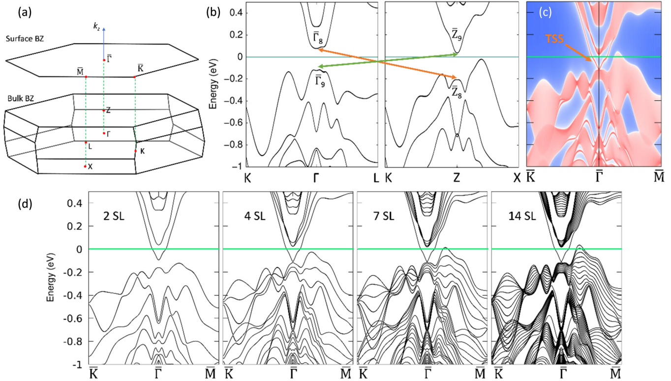
FIG. 5. (a) The BZ of \text{SnBi}_2\text{Te}_4 . (b) The calculated band structure of bulk \text{SnBi}_2\text{Te}_4 along the K\bar{\Gamma}L and KZX directions and showing the band inversion (green and orange lines). (c) The projection of the Brillouin zone along the \bar{K}\bar{\Gamma}\bar{M} direction and (d) the band structure of two, four, seven, and 14 SLs.
