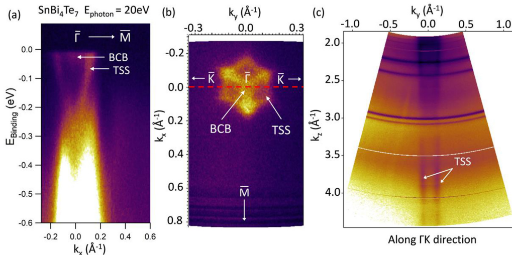
FIG. 6. (a) ARPES spectra of \text{SnBi}_4\text{Te}_7 for photon energy E_{\text{photon}} = 20 \text{ eV} along \bar{\Gamma}\bar{M} and (b) the Fermi surface of the same sample. (c) The photon energy dependent k_z - k_y Fermi surface map at E_F ( k_y parallel to \bar{\Gamma}\bar{K} ). The traces of the topological surface states (TSS) are recorded at the k_y values at which the dashed red line in (b) cuts the trace of the surface state. BCB denotes the bulk conduction band states.
