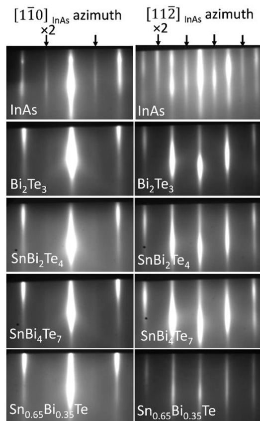
FIG. 1. RHEED patterns of \text{InAs}(111) substrate and Sn-Bi-Te films along the \text{InAs} [1 \bar{1} 0] and [1 1 \bar{2}] azimuths.
