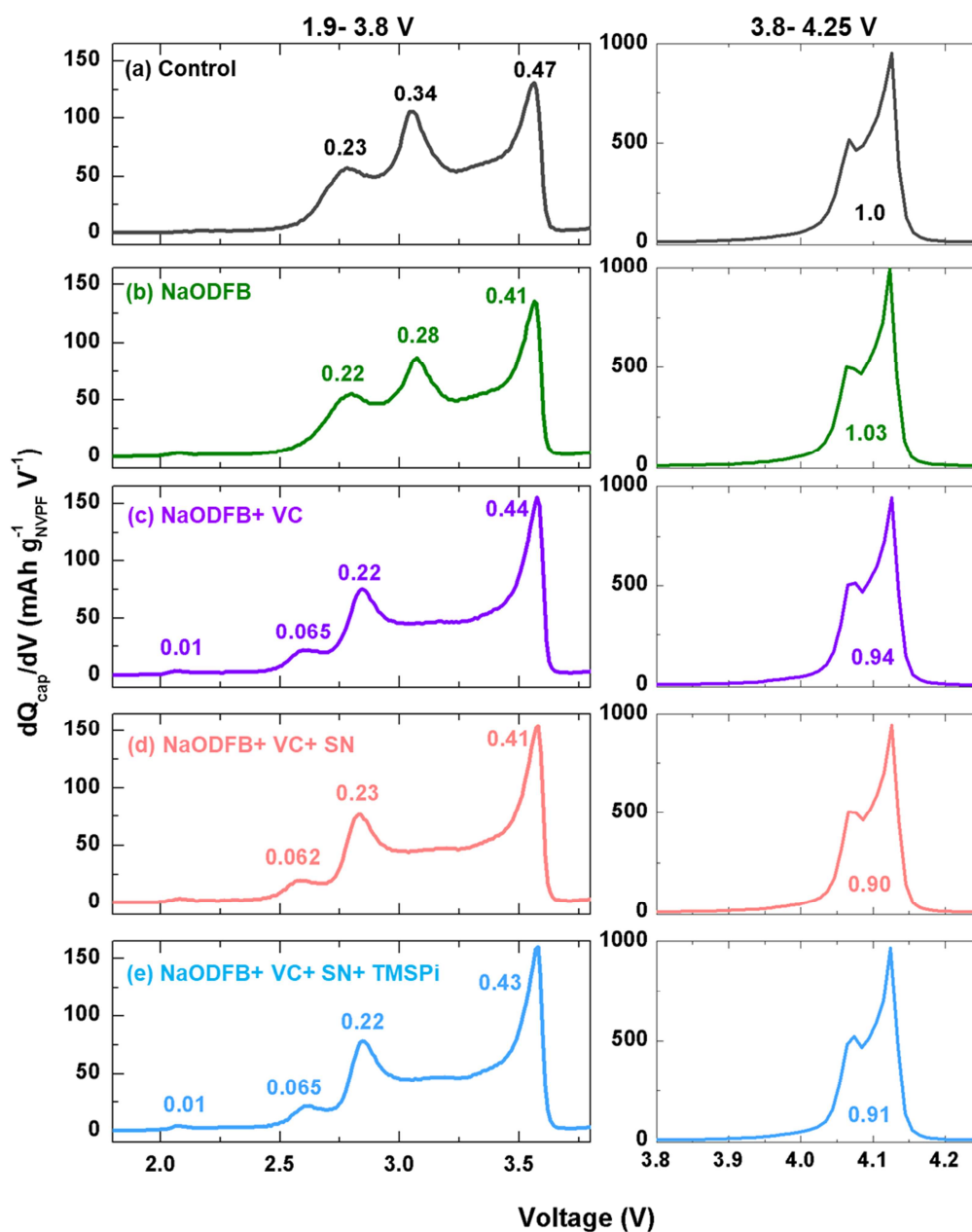
Figure S5. Capacity derivative dQ_{cap}/dV vs. voltage (V) plots for the 1 st charge of the NVPF/HC cylindrical 18650 cells. The voltage region from OCV- 3.8 V are shown in left and 3.8- 4.25 V in right. The electrolyte studied are the control electrolyte (1 M NaPF 6 in EC- PC- DMC 1: 1: 1 by volume) with no additive or having additives namely 0.5 wt% NaODFB, 0.5 wt% NaODFB+ 3 wt% VC, 0.5 wt% NaODFB+ 3 wt% VC+ 3 wt% SN and 0.5 wt% NaODFB+ 3 wt% VC+ 3 wt% SN+ 0.2 wt% TMSPi respectively. Amount of e - involved in the reaction corresponding to a particular peak is presented in the figure and is calculated with respect to NVPF. (Related to Figure 2)
