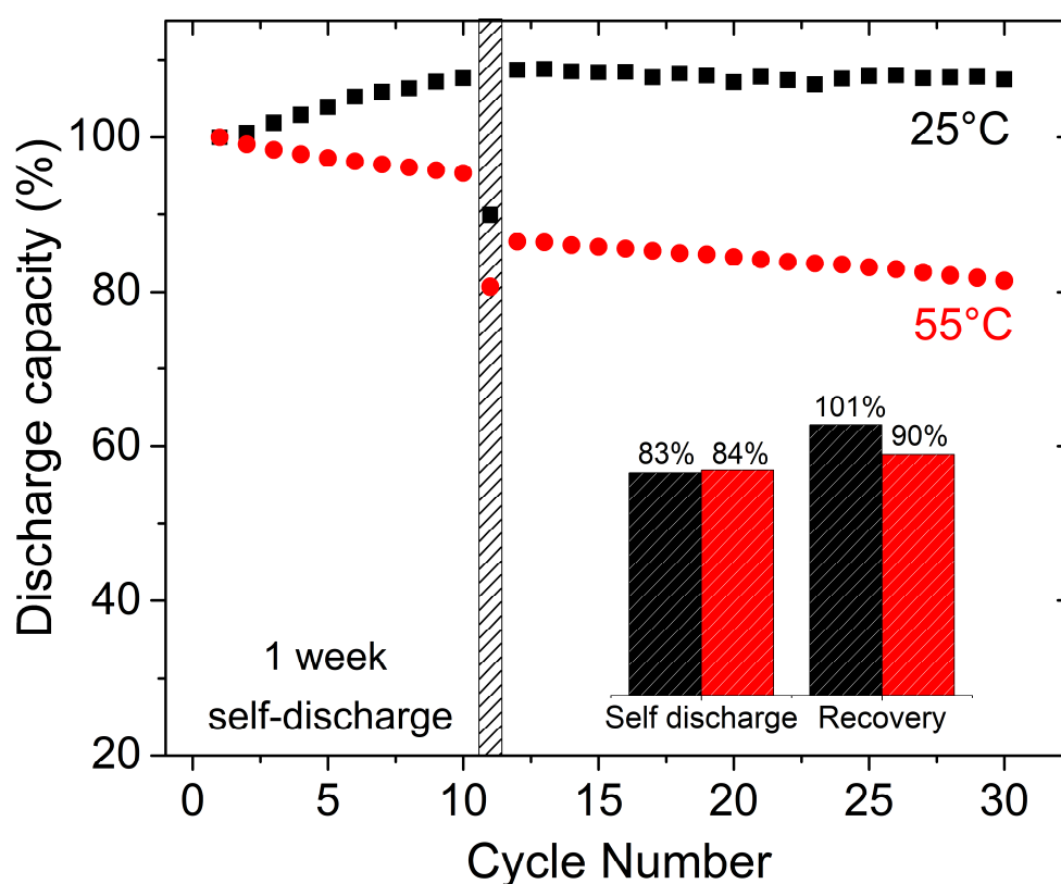
Figure S1. The percentage capacity retention vs. cycle number for Na 3 V 2 (PO 4 ) 2 F 3 (NVPF) / hard carbon (HC) full cells using 1M NaPF 6 in EC: PC: DMC (1:1:1 by volume) as electrolyte. The cells were cycled at C/5 in a fixed temperature of 25°C and 55°C by keeping them in an oven maintained at the required temperature. The cells were cycled for 10 cycles after which allowed to rest (self-discharge test) at 100% SOC (4.3V) for 1 week. Discharge capacity of 10 th , 11 th and 12 th cycle is Q 10 , Q 11 and Q 12 respectively. The percentage capacity observed just after self-discharge (Q 11 /Q 10 ) and in recovery cycle (Q 12 /Q 10 ) is presented in the histogram as inset in the Figure S1. Stable capacity retention with 100 % recovery was observed at 25 °C, while pronounced capacity decay with solely 90 % recovery after self-discharge test was obtained at 55 °C indicating the comparatively poor performance of the electrolyte at high temperature cycling.
