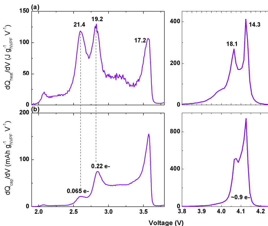
Figure S7. Comparison of derivative heat ( dQ_{\text{heat}}/dV ) with derivative capacity ( dQ_{\text{cap}}/dV ) as a function of potential (V) for the NVPF/HC cylindrical 18650 cells using 1M \text{NaPF}_6 in EC- PC- DMC (1: 1: 1 by volume) with additives NaODFB+ VC. The cells were cycled at 55°C using C/10 rate. The total heats (in joules per gram of NVPF) for each exothermic peak were measured by integrating the total area under the peak and are mentioned in (a). Similarly, the corresponding electrons involved were measured from the capacity obtained in that voltage region and converting them to \Delta\text{Na} , hence electrons ( e^- ). The heat evolution peaks at 2.6 V and 2.8 V have almost similar area but the corresponding e^- involved at 2.6 V are less than that at 2.8 V, indicating the process at 2.6 V is highly exothermic chemical/ electrochemical reaction. (Related to Figure S2c)
