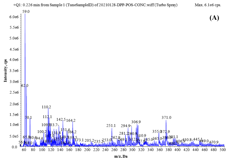
Fig. 2 : Full scan mass spectra in the m/z 50-500 range of DPhP in positive (A) and negative (B) ionization mode, MS/MS mass spectrum of the [M - H] - ion (m/z 249) of DPhP (C) with -40 V collision energy.
