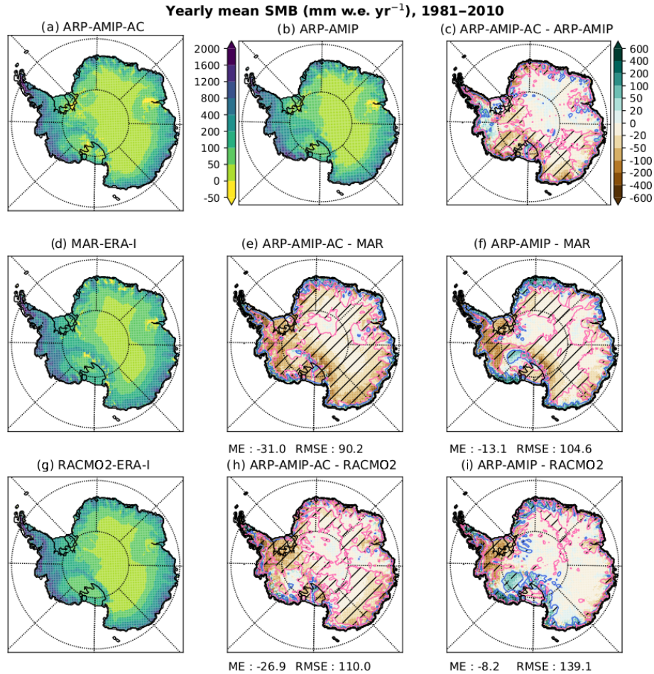
Figure 6. Yearly mean total SMB (mm w.e. yr -1 ) for ARP-AMIP-AC (a), ARP-AMIP (b), MAR-ERA-I (d) and RACMO2-ERA-I (g) for the reference period 1981–2010. Difference (mm w.e. yr -1 ) for ARP-AMIP-AC minus ARP-AMIP (c), ARP-AMIP-AC minus MAR-ERA-I (e), ARP-AMIP minus MAR-ERA-I (f), ARP-AMIP-AC minus RACMO2-ERA-I (h) and ARP-AMIP minus RACMO2-ERA-I (i). Blue (magenta) hatched contour lines represent areas where the positive (negative) difference is larger than 20 %. Mean error (ME) and RMSE statistics (mm w.e. yr -1 ) for the comparison with MAR and RACMO2 are shown below the panel.
