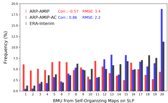
Figure 3. Best-matching-unit (BMU) relative frequency (%) of ARP-AMIP (red), ARP-AMIP-AC (blue) and ERA-I (black) on daily SLP map over the 1981–2010 period. Root mean square errors and Pearson correlation coefficient with respect to ERA-I BMU frequencies are shown to the right of the legend.
