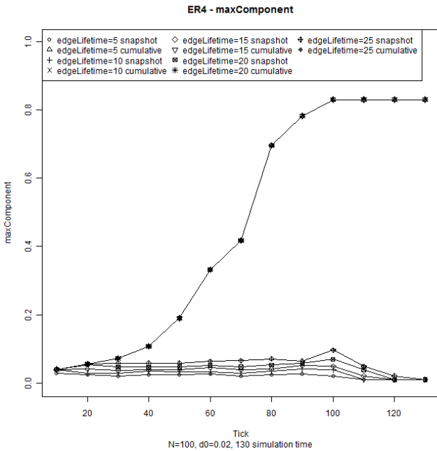
Figure 7: ER4 Fractional Size of the Maximal Component
