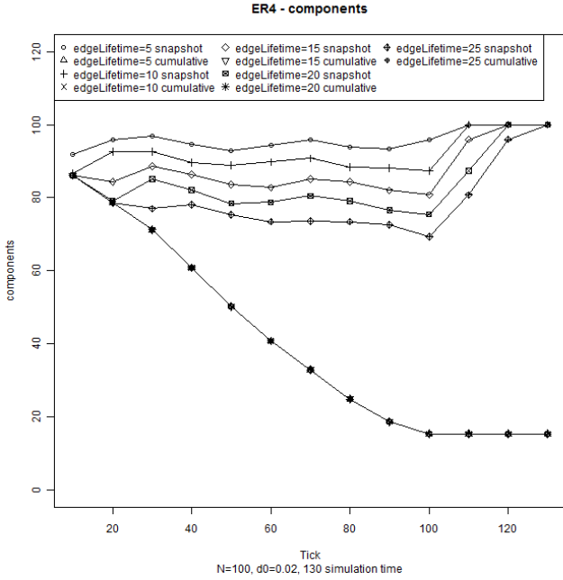
Figure 6: ER4 Components
