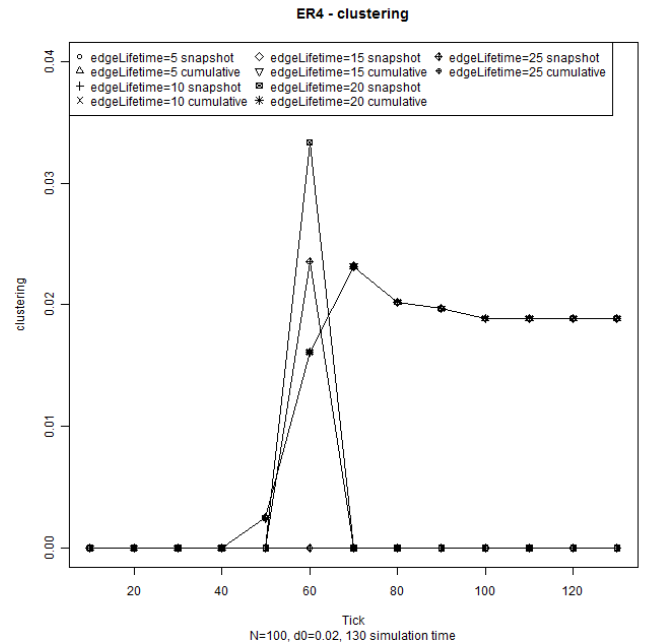
Figure 5: ER4 Clustering
