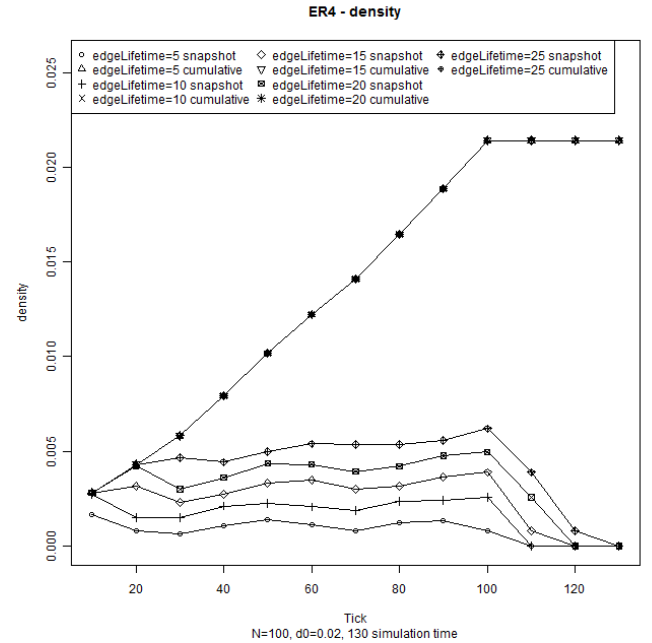
Figure 2: ER4 Density
