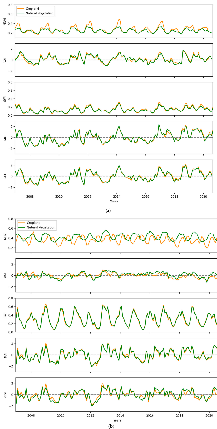
Figure 10. NDVI, SWI, VAI, MAI, and GDI time series at two test sites (a) Kairouan and (b) Andalusia.
