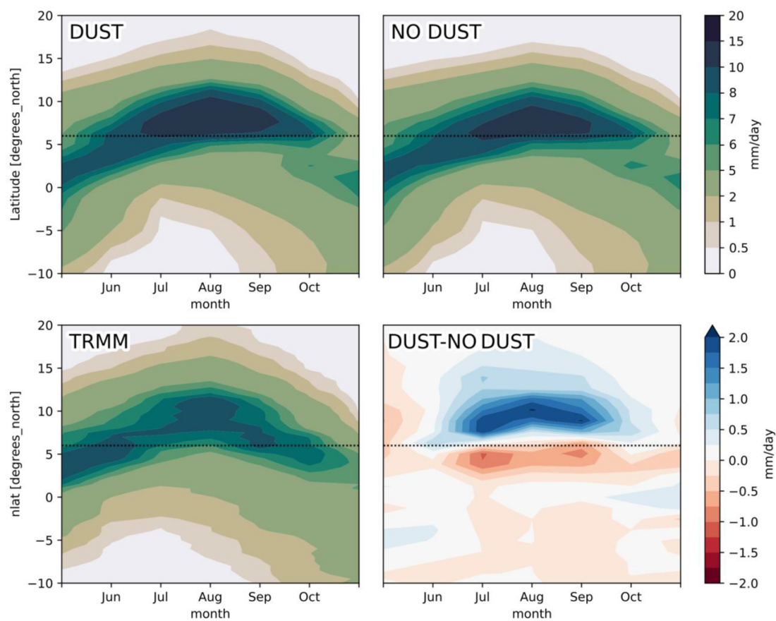
Figure 5. A Hovmöller diagram showing the time and latitudinal variations in the zonally averaged precipitation (millimeters per day) from 10° W to 10° E from 2000 to 2014. The TRMM indicates the observed precipitations from the NASA Tropical Rainfall Measuring Mission.
