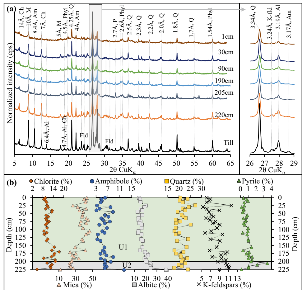
Fig. 3 a XRD patterns of bulk sediments. Ch, chlorite; M, mica; Am, amphibole; Phyl, phyllosilicates; Q, quartz; P, pyrite; Fld, feldspars; K-fld, K-rich feldspars (orthoclase and microcline); and Al, albite. The inset to the right highlights the change in quartz and feldspar peaks. b Mineral contents of the bulk sediments as a function of depth
