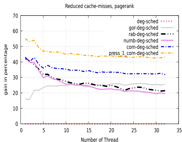
Figure 16: cache-misses with scheduling – Orkut
