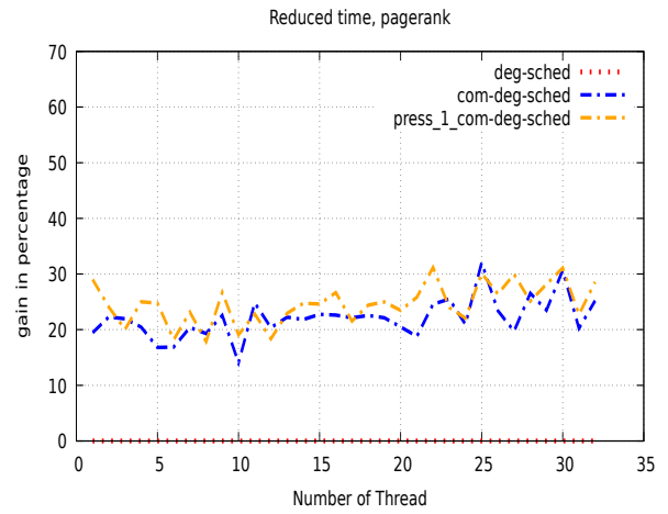
Figure 24: time reduced with scheduling – Lj
