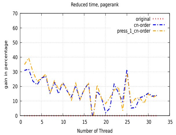
Figure 26: time reduced with graph orders – Orkut
