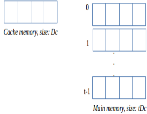
Figure 4: Memory representation
