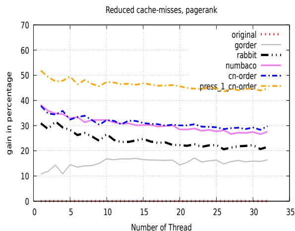
Figure 18: cache-misses with graph orders – Lj
