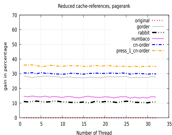
Figure 6: cache-ref with graph orders – Orkut
