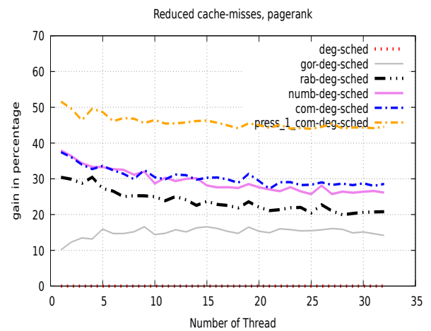
Figure 20: cache-misses with scheduling – Lj
