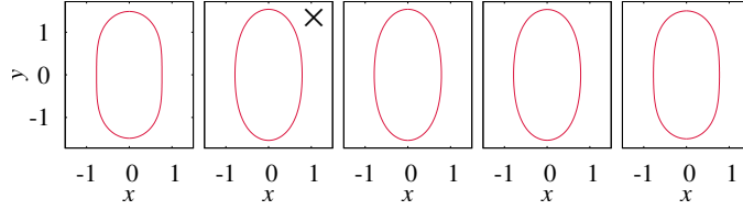
FIG. 15. Observed shapes in the deformation of a vesicle in UP(t_m) at \beta = 2.0 and \sigma_r = 10 . Shapes correspond to t = 0, 0.6^\times, 0.65, 1.0, \text{ and } 18.0 .
