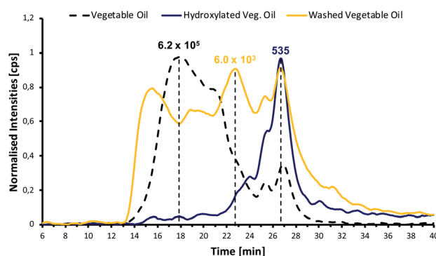
Fig. 3 GPC-ICP-MS chromatogram of the vegetable oil, washed vegetable oil at basic pH, and hydroxylated vegetable oil samples. The numbers on top of the peaks represent the estimated molecular weight [Da] of the eluting species.
