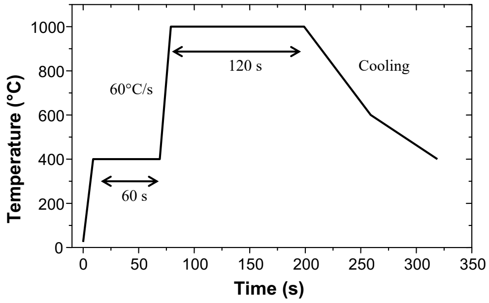
Figure 2. Annealing profile
