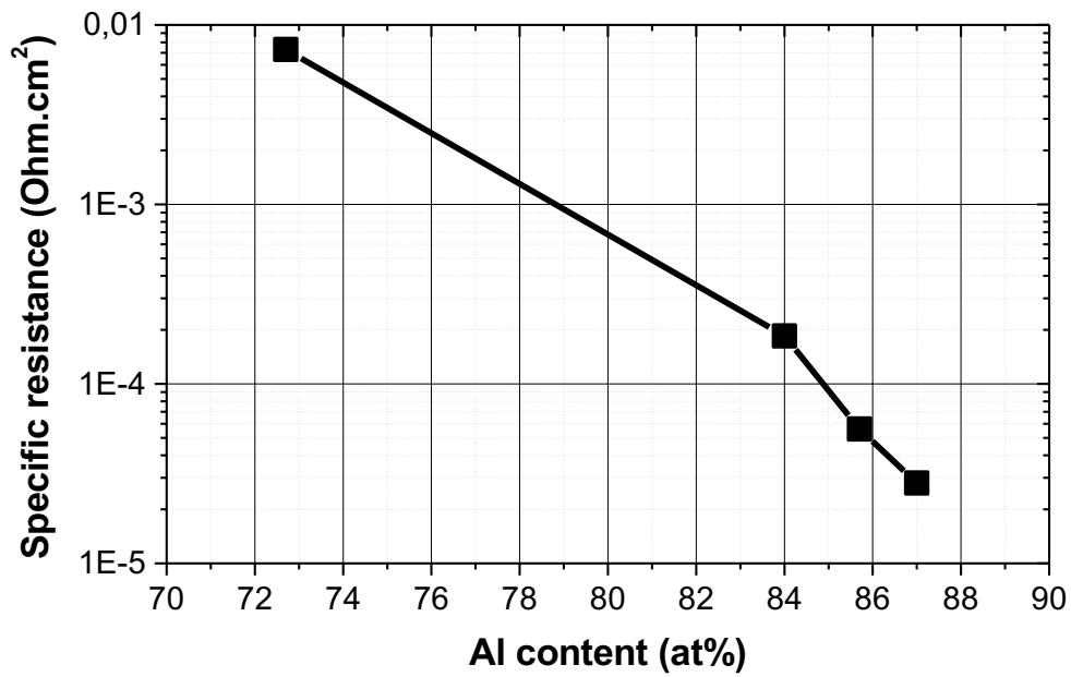
Figure 1. Specific resistance versus the Al content in the contact.
