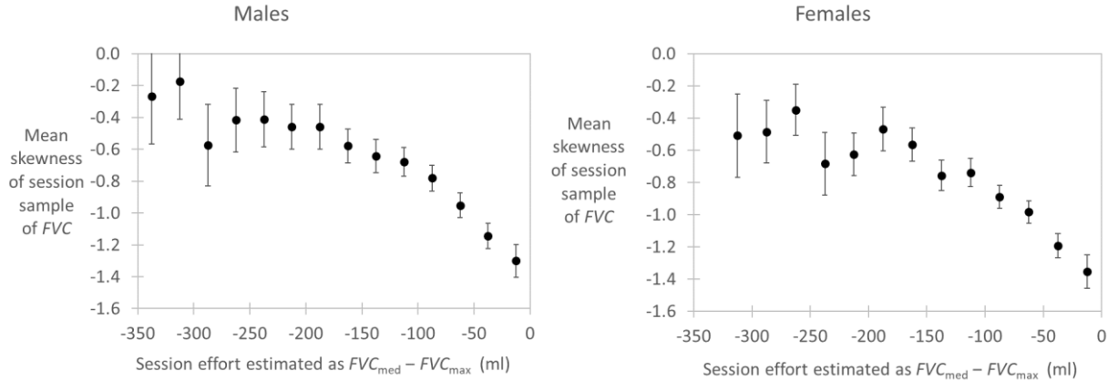
Figure 4. Session skewness of FVC as a function of session effort, computed as FVC_{med} - FVC_{max} . Each data point corresponds to one specific effort group where that difference, represented on the horizontal axis, falls within an interval of 25 ml (e.g., from 100 to 125 ml). Error bars represent 95% confidence limits.
