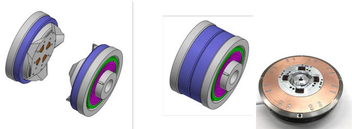
Figure 8: HOTDOCK interface concept before and after coupling
