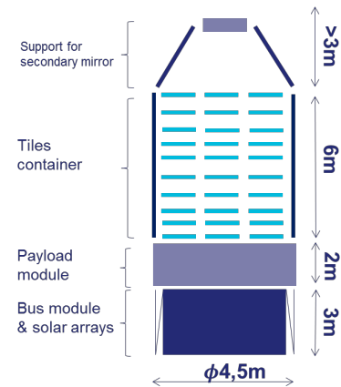
Figure 4: Sizing configuration
