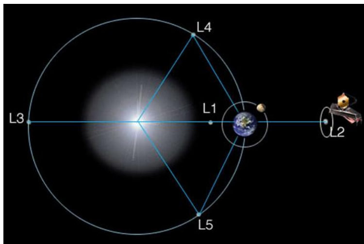
Figure 2: Sun-Earth Lagrangian points (Courtesy of NASA)
