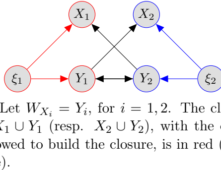
Figure 3: Topological separation is easy to check: nonrecursive system.
