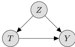
(a) Common cause example.
