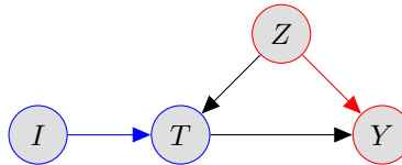
(b) Modeling intervention with the intervention variable I .
