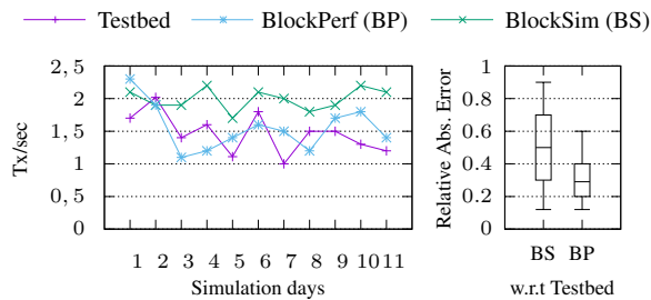
Figure 17: Throughput (o) & relative absolute error w.r.t Testbed
