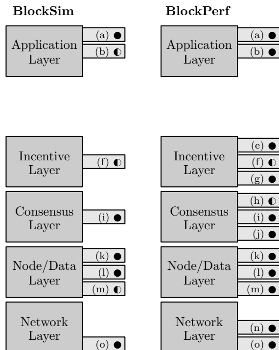
Figure 3: Illustration of how BlockPerf extends BlockSim - ● symbol indicates that the simulator makes available the performance metric without any code modification and/or post-processing, while ◐ symbol indicates that such a modification and/or post-processing is needed to obtain the desired performance metric
