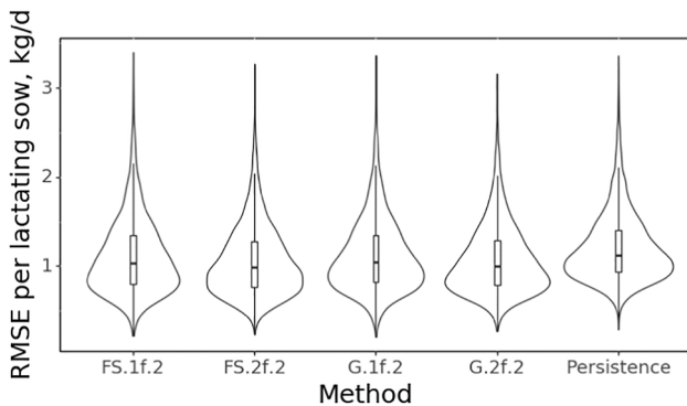
Fig. 7. Root Mean Square Error (RMSE) per lactating sow according to the combination of learning methods (FS: Farm Specific; G: Global) and forecasting functions (1f,2f) with two clusters ( k = 2 ), and without learning with the Persistence forecasting function.
