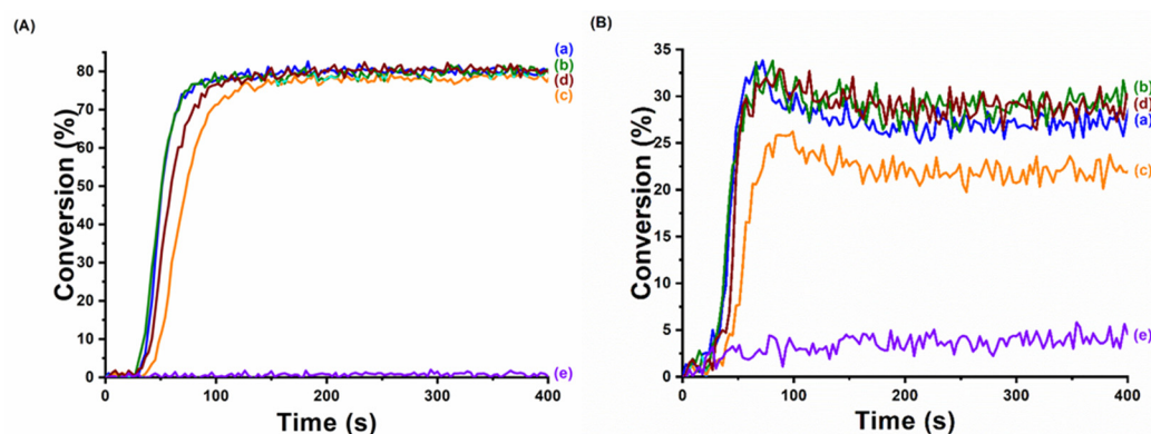
Figure 18. Polymerization profiles (A) (acrylate function conversion vs. irradiation time) and (B) (epoxide function conversion vs. irradiation time) of TMPTA/EPOX blend (50/50 w/w %) upon irradiation with a LED at 530 nm, under air, sample thickness = 1.4 mm; the irradiation starts at 10 s, 11 \text{ mW cm}^{-2} . Photoinitiating systems: (curve a) Cu1BF 4 /Iod/EDB (0.70/2.0/2.0 w/w/w %), (curve b) Cu1PF 6 /Iod/EDB (0.70/2.0/2.0 w/w/w %), (curve c) Cu2BF 4 /Iod/EDB (0.63/2.0/2.0 w/w/w %), (curve d) Cu2PF 6 /Iod/EDB (0.64/2.0/2.0 w/w/w %) and (curve e) Iod/EDB (2.0/2.0 w/w %).
