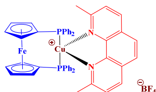
Figure 5. Chemical structure of \text{Cu3BF4} .
