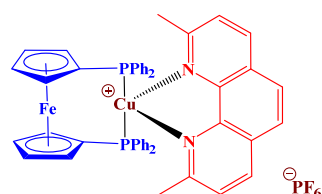
Figure 6. Chemical structure of \text{Cu3PF6} .
