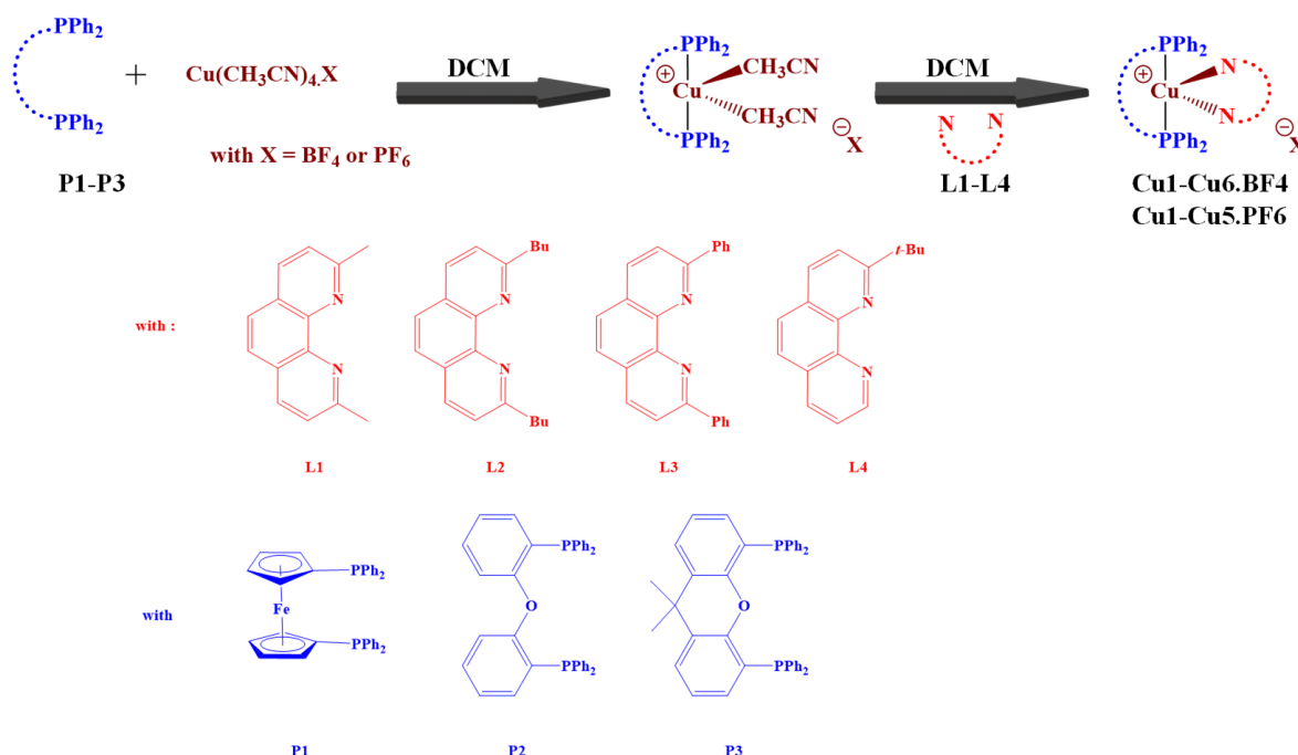
Scheme 2. Synthetic routes to \text{Cu1-Cu6.BF}_4 , \text{Cu1-Cu5.PF}_6 .
