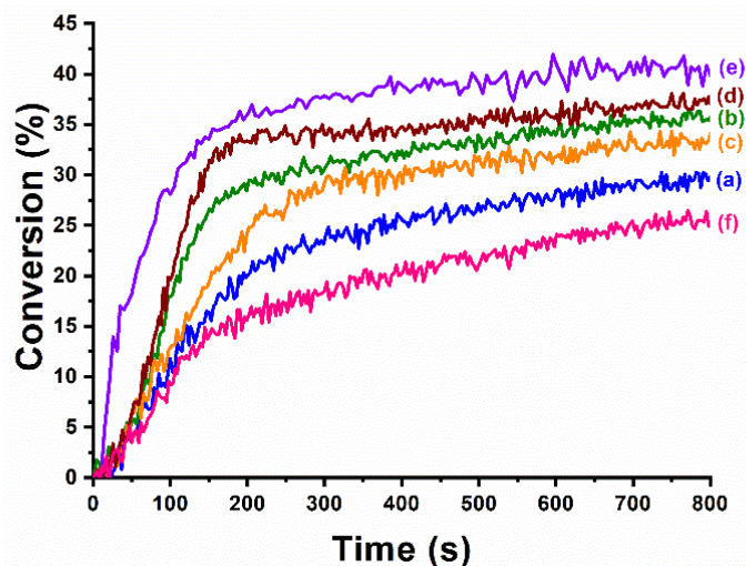
Figure 15. Polymerization profiles (epoxide function conversion vs. irradiation time) of EPOX upon irradiation with a LED at 405 nm, under air, sample thickness = 1.4 mm; the irradiation starts at 10 s, 50 mW cm -2 . Photoinitiating systems: (curve a) Cu1BF4/Iod/EDB (0.72/2.0/2.0 w/w/w%), (curve b) Cu1PF6/Iod/EDB (0.68/2.0/2.0 w/w/w%), (curve c) Cu2BF4/Iod/EDB (0.61/2.0/2.0 w/w/w%), (curve d) Cu2PF6/Iod/EDB (0.63/2.0/2.0 w/w/w%), (curve e) G1/Iod/EDB (0.33/2.0/2.0 w/w/w%) and (curve f) Iod/EDB (2.0/2.0 w/w%).
