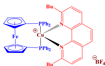
Figure 7. Chemical structure of Cu4BF4.
