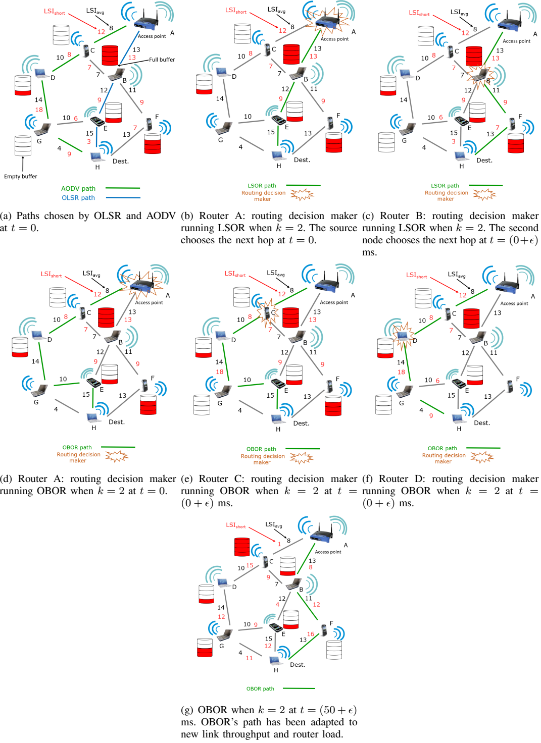
Fig. 2: An example of the paths chosen by OLSR, AODV, LSOR and OBOR when k = 2 .
