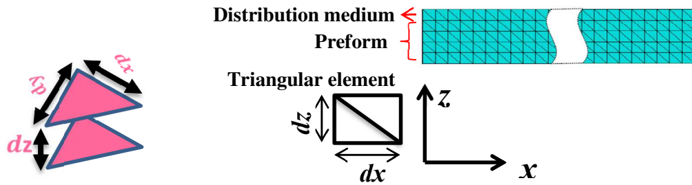
Figure 4(b) Element size definitions in multi-layered shell element (left) and in 2D shell element (right) Figure 4. Definition of the flow condition and of the element dimensions for the 3D simulation by multi-layered shell elements and for the 2D simulation by shell elements
