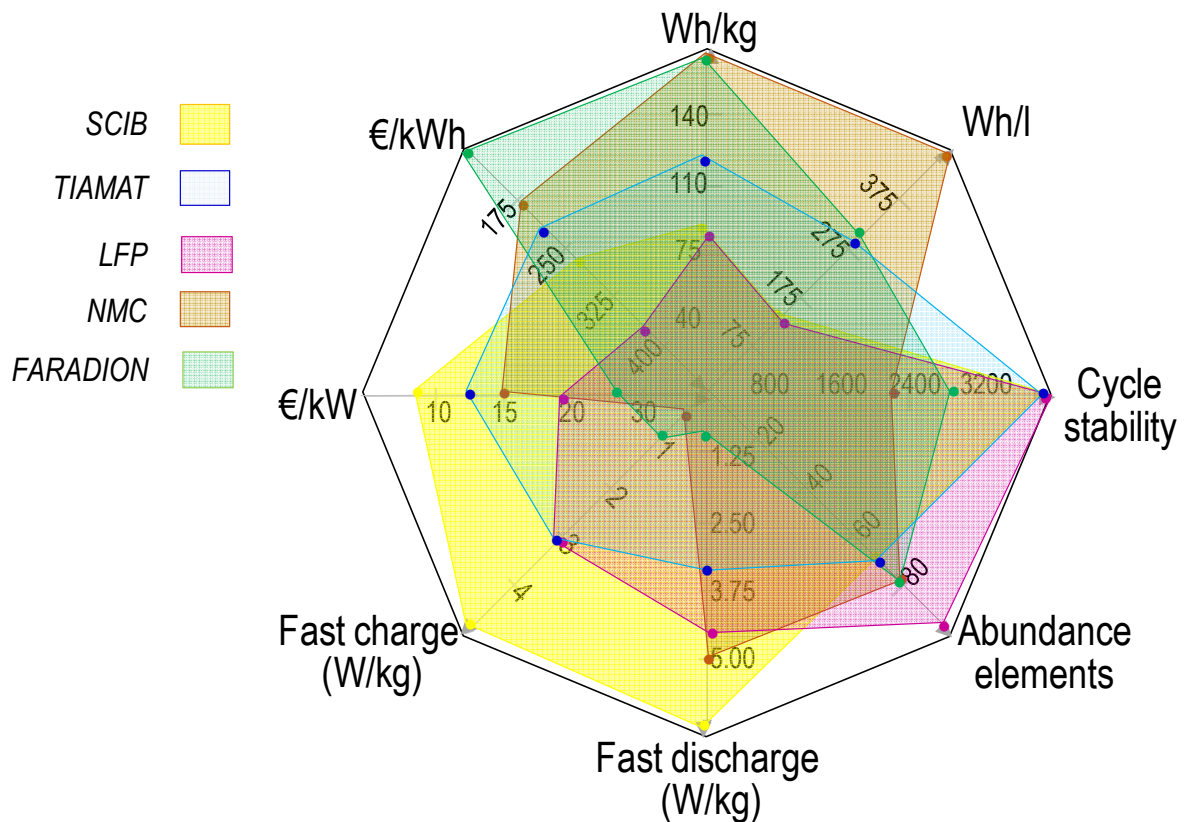
Figure 2: Tentative comparison between high power cells relying on either Na-ion technology NVPF/C 18650 or \text{Na}_x\text{MO}_2/\text{C} pouch cells) or on the Li-ion technology LFP/C (18650) , NMC/C and SCIB pouch cells. Several trends are conveyed from the reported figures of merit deduced from open reports.. The NVPF/C Na-ion system overrides the \text{Na}_x\text{MO}_2/\text{C} in terms power rate with this ranking be reversed when autonomy is considered. Moreover, NVPF/C compares favorably to LFP for nearly all the figures of merit, but it falls short against SCIB in terms of power while less costly in €/kWh and more performing in Wh/kg and Wh/l. Lastly, turning to the importance of qualifying the \text{W/kg}_{\text{charge}} and \text{W/kg}_{\text{discharge}} for power application, note that the largest difference is for the Li-NMC chemistry. Obviously, not a single technology meet all the figures of merit at one, but NVPF/C is performing the bests for applications conjugating high power with a correct degree of autonomy. (With the courtesy of M; Morcrette).
