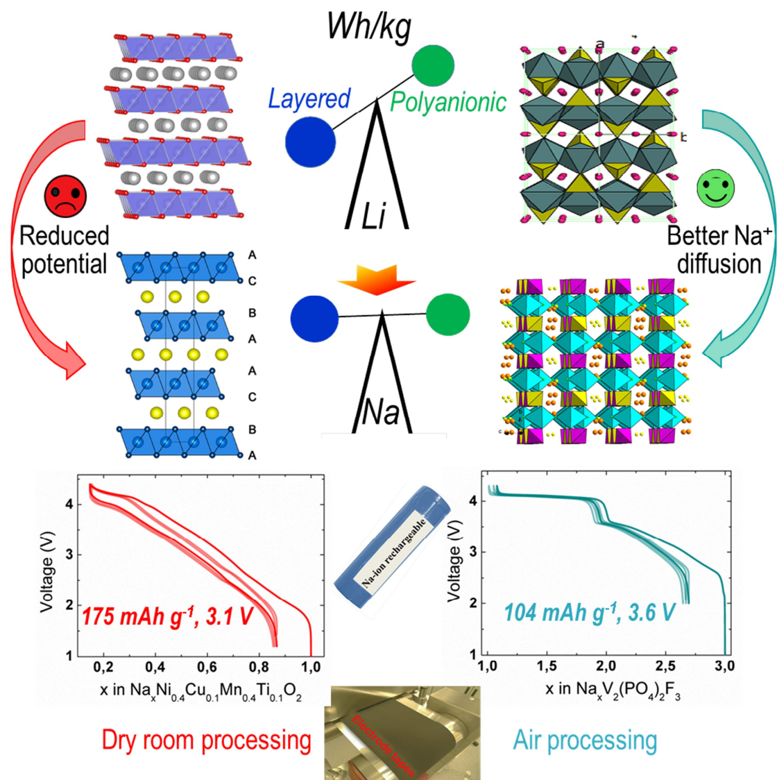
Figure 1: Comparison of both Li and Na-ion technology that share the same family of layered and polyanionic compounds. Power-wise, the supremacy of the latter over the former is enhanced by switching from the Li to Na-ion technology, while the large gain in energy density provided by layered skeletons over polyanionic ones is strongly reduced owing to a diminution of the Na-redox potential in layered oxide. This leads to a lower output cell voltage but also implies the need of handling-processing of the electrode in a moisture-free environment. Some issues can be mitigated by realizing O3-P2 composites or by proper substitution of O3 skeletons to the expense of a lower capacity performance (with the courtesy of S. Mariyappan).
