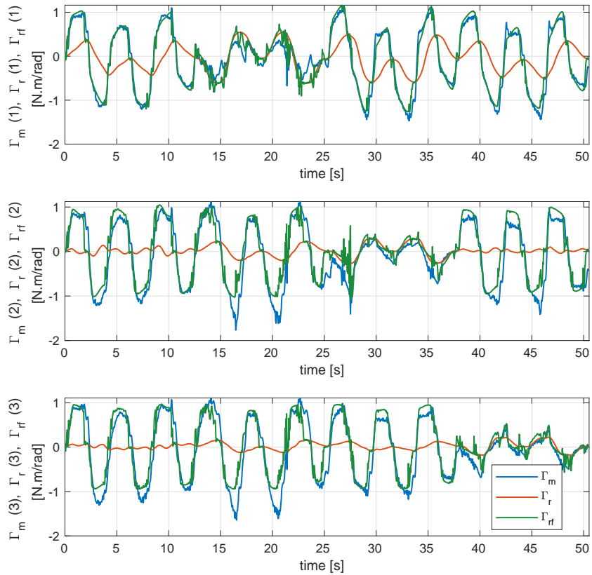
Fig. 4: Time history of torques calculated from the dynamic model with friction ( \Gamma_{rf} , green plot), without friction ( \Gamma_r , red plot) and calculated from motor forces ( \Gamma_m , blue plot).
