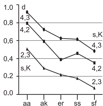
Fig. 1. Average damage size for different network types: aa -aggregate of automata k = K , Kauffman networks: ak -( k = K ), er -random Erdős-Rényi network, ss -single-scale and sf -scale-free; and different parameters s, K=4,3; 4,2 and 2,3 . Note that for 4,2 and 2,3 the coefficient w = 1.5 . We cannot limit ourselves to one of K, s and w parameters or one network type. The shown points have 3 decimal digits of precision. These networks are autonomous, they are built without adaptive condition. The er network is the only one with k = 0 .
