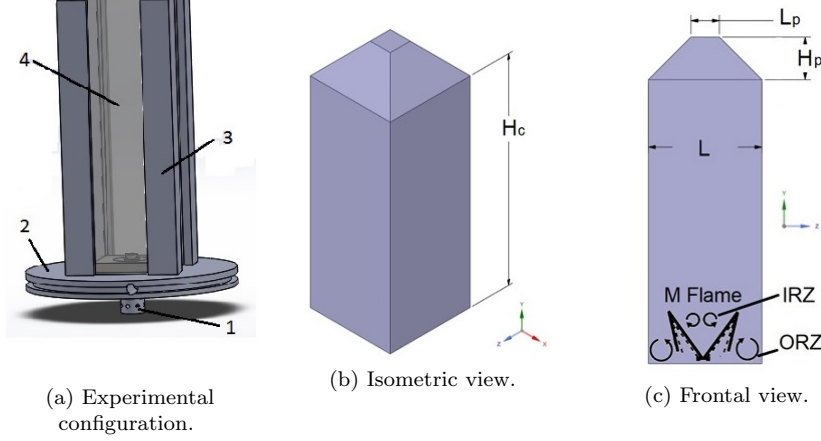
Fig. 1 Combustion chamber schematic view. In the experimental configuration: 1 swirler, 2 cooling base, 3 confinement, 4 quartz window, adapted from [26].
