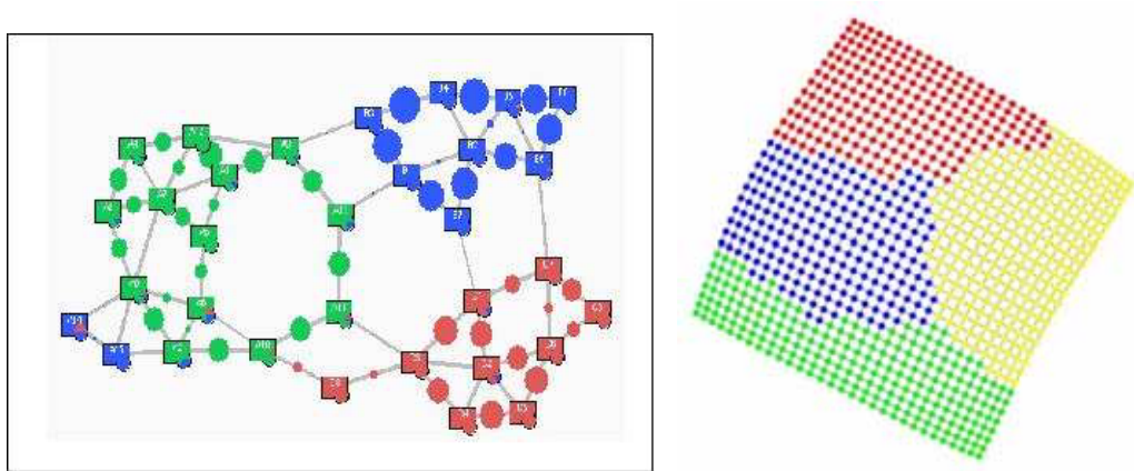
Figure 3: AntCo2 algorithm for graph clustering: on the left the output of the computation on a communication network; on the right the output on a regular grid
