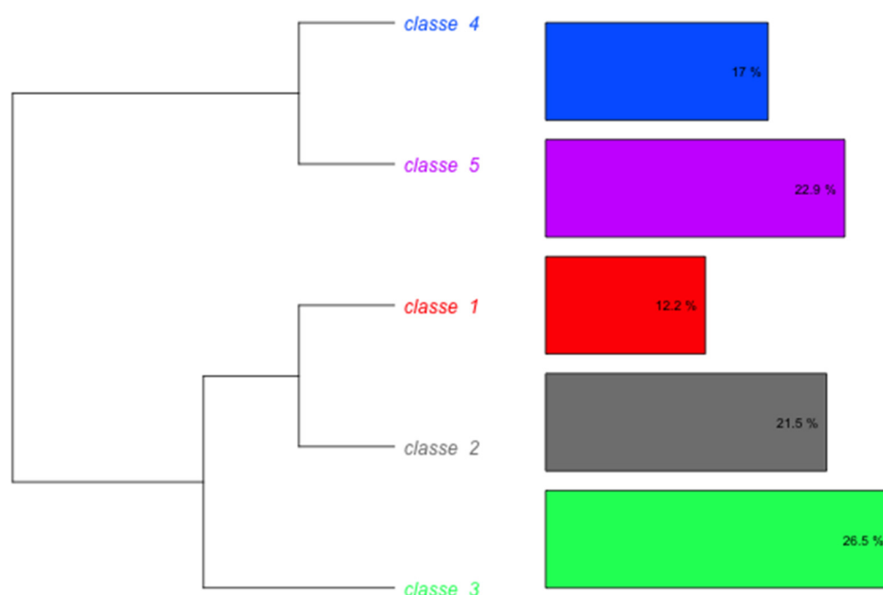
Figure 3. Dendrogram—first interview—parents.
