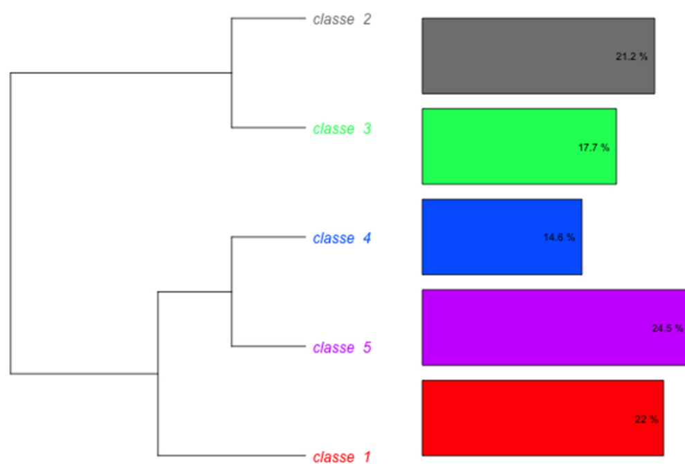
Figure 1. Dendrogram—parental corpus.
