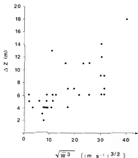
Fig. 8. Vertical excursion plotted against \sqrt{W^3} , where \Delta Z is the depth at which the profile of \Delta R changed slope to become approximately parallel to G
