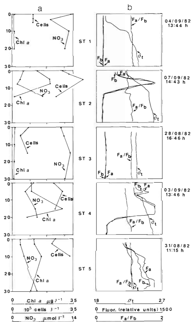
Fig. 1. Typical profiles of (a) total cell numbers, chlorophyll a and \text{NO}_3 , and (b) \sigma_t , fluorescence before ( F_b ) and after ( F_a ) exposure to bright light, and the ratio R = F_a/F_b . Time and date of sampling are indicated on the right for each station
