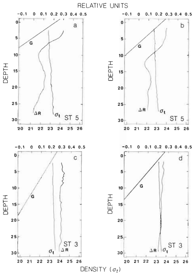
Fig. 9. Typical examples of profiles of \Delta R , G and \sigma_t
