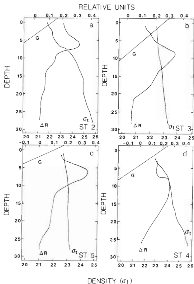
Fig. 6. Typical examples of profiles of \Delta R , G and \sigma_t showing photoinhibition
