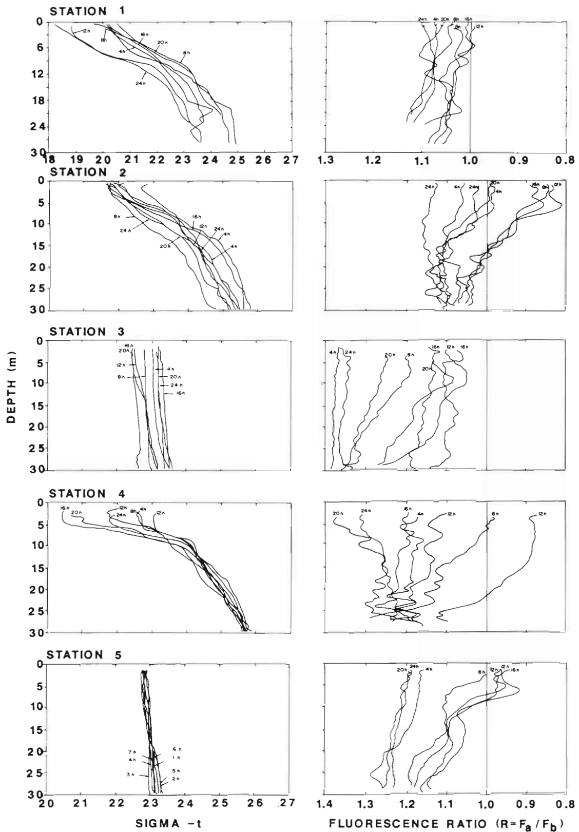
Fig. 2. Time series of vertical profiles of \sigma_t and fluorescence ratio at the 5 stations in the St. Lawrence Estuary
