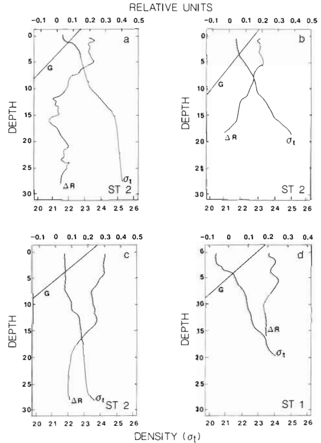
Fig. 5. Typical examples of profiles of \Delta R , G and \sigma_t
