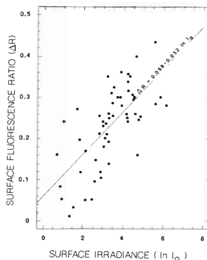
Fig. 3 Scatter diagram for the combined values of the surface fluorescence ratio and the logarithm of irradiance
