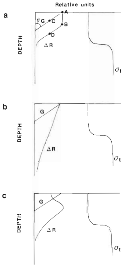
Fig. 4. Conceptual model of the vertical responses of the fluorescence ratio R = F_a/F_b to changes in irradiance and stratification
