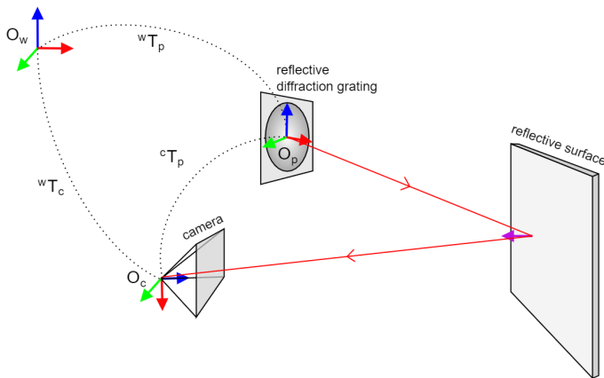
Fig. 2: Coordinate systems of objects of the system.
