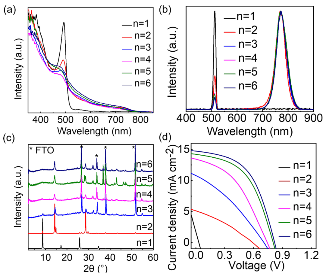
Figure 6. Film properties of (\text{mPDA})\text{MA}_{n-1}\text{Pb}_n\text{I}_{3n+1} ( n = 1-6 ), (a) UV-Vis absorption spectra, (b) steady-state PL spectra, the first peak at 512 nm showing the n = 1 phase, the second emission peak at 773 nm showing the 3D bulk phase. (c) PXRD patterns, and (d) J - V curves of devices.
