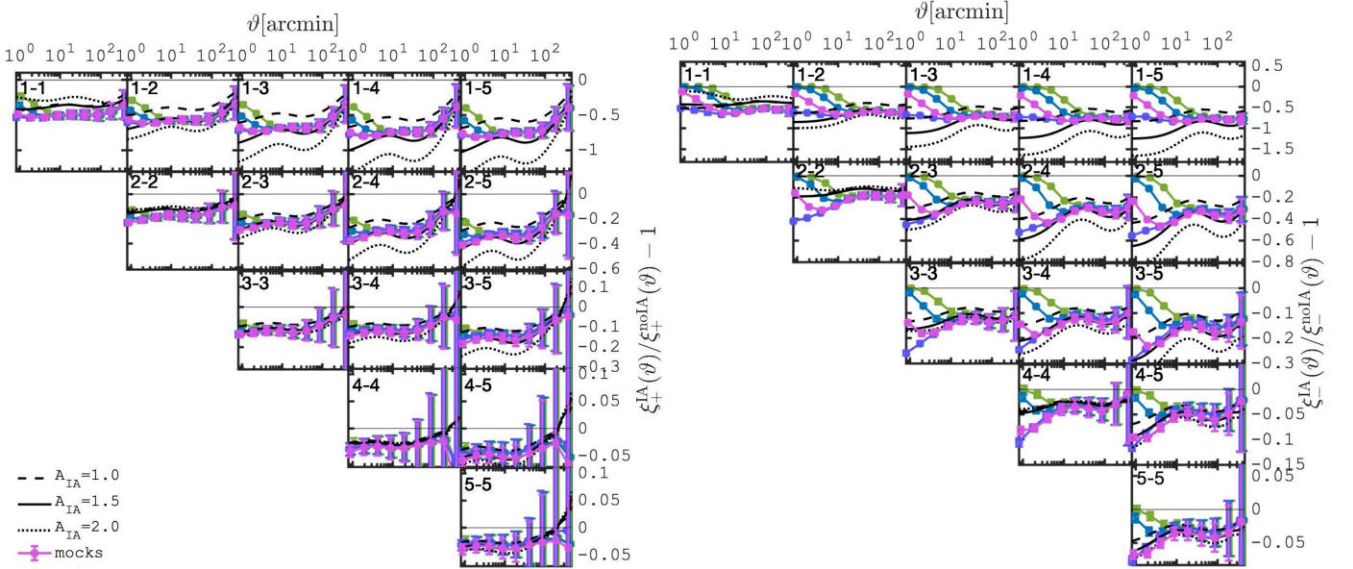
Figure 4. Fractional difference between the shear 2PCFs with and without the IA signal, \xi_{\pm}^{IA} / \xi_{\pm}^{noIA} - 1 , in the NLA model. The theory lines show the predictions with three values of the A_{IA} parameter indicated in the legend, while the measurements are for A_{IA} = 1.5 with different smoothing scales: the magenta squares are our default model, with \sigma_G = 0.1 h^{-1} Mpc, while the other coloured curves show \sigma_G = 0.5 (green), 0.25 (blue), and 0.0 h^{-1} Mpc (purple). The error bars show the error on the mean measured from 50 light cones. Note the different scaling of the y-axis. As for Fig. 3, no shape noise is included in this figure, to better exhibit the IA signature. The thin horizontal line represents the A_{IA} = 0.0 case.
