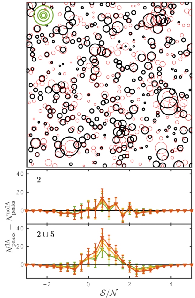
Figure 8. (upper:) Position and height of the peaks measured in the tomographic bin combination 2U5, with A_{\text{IA}} = 2.0 (red) and 0.0 (black), inside a 1.0 \text{ deg}^2 patch. The four concentric circles indicate the sizes for S/\mathcal{N} = 1, 2, 3 and 4. (lower:) Difference between the peak function with and without IA as measured from our 50 KiDS-like catalogues, for the tomographic bin 2 and the combination 2U5, shown for A_{\text{IA}} = 1.0 (green), 1.5 (yellow) and 2.0 (orange).
