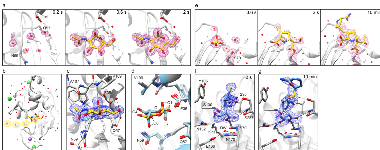
Fig. 2 Drop-on-drop delivery enables the analysis of N-acetyl-D-glucosamine (GlcNAc) binding to the HEWL active site and catalytic activity of CTX-M-15 by serial X-ray crystallography. a 2mF_o-DF_c electron density maps for HEWL-GlcNAc XFEL structures, displayed at \pm 1\sigma contour level and carved at 2\text{ \AA} around the GlcNAc ligand. The GlcNAc molecule from the 2 s time point structure was used to carve the 200 ms time point map. All maps are at 1.45\text{ \AA} resolution. b Cartoon representation of the HEWL structure (2 s mixing time point, PDB ID 7BHN). GlcNAc is shown as sticks and colored in yellow. Waters, sodium, and chloride ions are shown as red, purple, and green spheres, respectively. Ligand binding subsites A-D (as in PDB ID 5NJR 10 ) are indicated by yellow circles. c, d Close-up active site view of the HEWL structure shown in (b) . c mF_o-DF_c polder OMIT difference density map contoured at \pm 3\sigma and carved 1.5\text{ \AA} around the ligand site. Hydrogen bonding network is highlighted. d Superimposition of the 2 s mixing time point structure (yellow and gray) and the single-crystal room-temperature structure of HEWL soaked with GlcNAc obtained by Tanley et al. 25 (light blue, PDB 3TXJ). e 2mF_o-DF_c electron density maps of CTX-M-15 structure displayed at \pm 1\sigma and carved at 2\text{ \AA} around the ertapenem ligand (pink; 1.55, 1.55, and 1.65\text{ \AA} for 0.6 s, 2, and 10 min, respectively). The 0.6 and 2 s time points are calculated with XFEL data, whereas the 10 min time point is calculated with room temperature, SSX data collected at Diamond Light Source. f, g Close-up view of the structure obtained after 2 s ( f ) and 10 min ( g ) of mixing with ertapenem. Interactions of ertapenem (blue sticks) with residues on the protein main chain (gray sticks) as well as the interactions of the proposed deacylating water (DW, red sphere) with the protein are shown as black dashes. mF_o-DF_c polder OMIT difference density maps are contoured at \pm 3\sigma and carved 1.5\text{ \AA} around the ligand site. Ertapenem has been tentatively modeled and refined into the observed electron density as the ( R )- \Delta^1 -pyrroline tautomer for both 0.6 s and 10 min structures (see Supplementary Note 3). Graphic was created using the UCSF Chimera package 54 .
